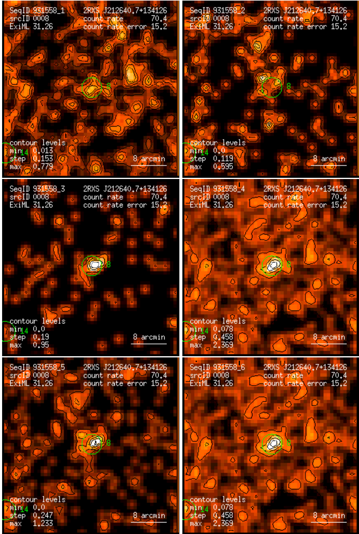
Figure 8: RASS 931558: detection 0008: band rate images, Gaussian filter: (1) PSPC channels 11 – 41, (2) 52 – 90, (3) 91 – 201, (4) 11 – 235, (5) 52 – 201, (6) 11 – 201. Broad band rates in counts/ks. Band rate contour levels in counts/ks/arcmin 2 .
