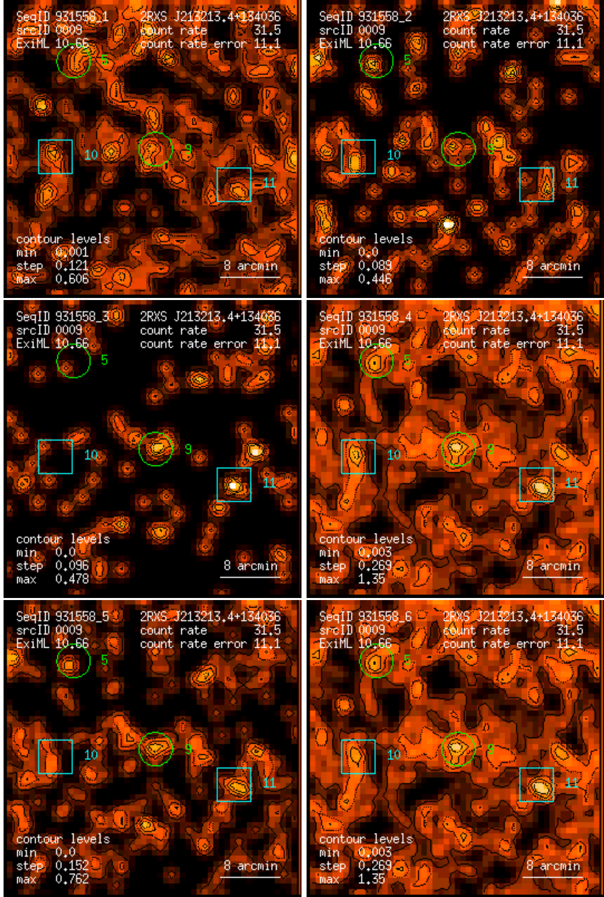
Figure 9: RASS 931558: detection 0009: band rate images, Gaussian filter: (1) PSPC channels 11 – 41, (2) 52 – 90, (3) 91 – 201, (4) 11 – 235, (5) 52 – 201, (6) 11 – 201. Broad band rates in counts/ks. Band rate contour levels in counts/ks/arcmin 2 .
