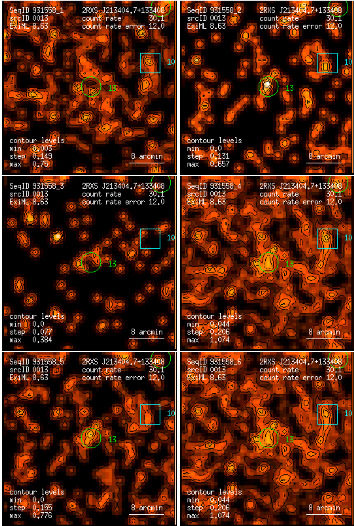
Figure 13: RASS 931558: detection 0013: band rate images, Gaussian filter: (1) PSPC channels 11 – 41, (2) 52 – 90, (3) 91 – 201, (4) 11 – 235, (5) 52 – 201, (6) 11 – 201. Broad band rates in counts/ks. Band rate contour levels in counts/ks/arcmin 2 .
