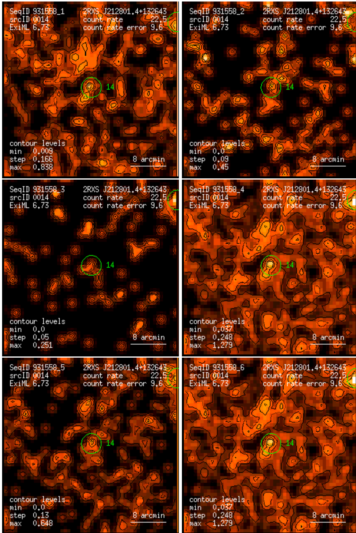
Figure 14: RASS 931558: detection 0014: band rate images, Gaussian filter: (1) PSPC channels 11 – 41, (2) 52 – 90, (3) 91 – 201, (4) 11 – 235, (5) 52 – 201, (6) 11 – 201. Broad band rates in counts/ks. Band rate contour levels in counts/ks/arcmin 2 .
