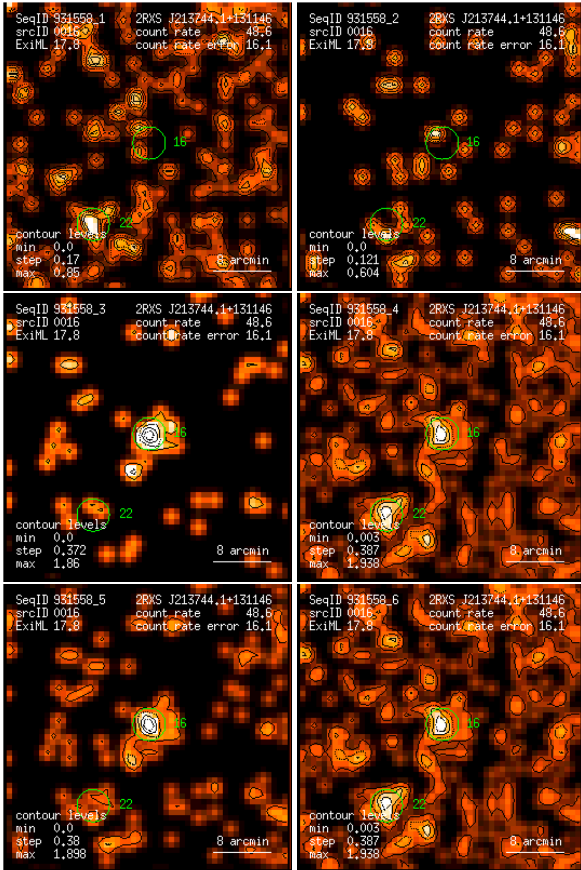
Figure 16: RASS 931558: detection 0016: band rate images, Gaussian filter: (1) PSPC channels 11 – 41, (2) 52 – 90, (3) 91 – 201, (4) 11 – 235, (5) 52 – 201, (6) 11 – 201. Broad band rates in counts/ks. Band rate contour levels in counts/ks/arcmin 2 .
