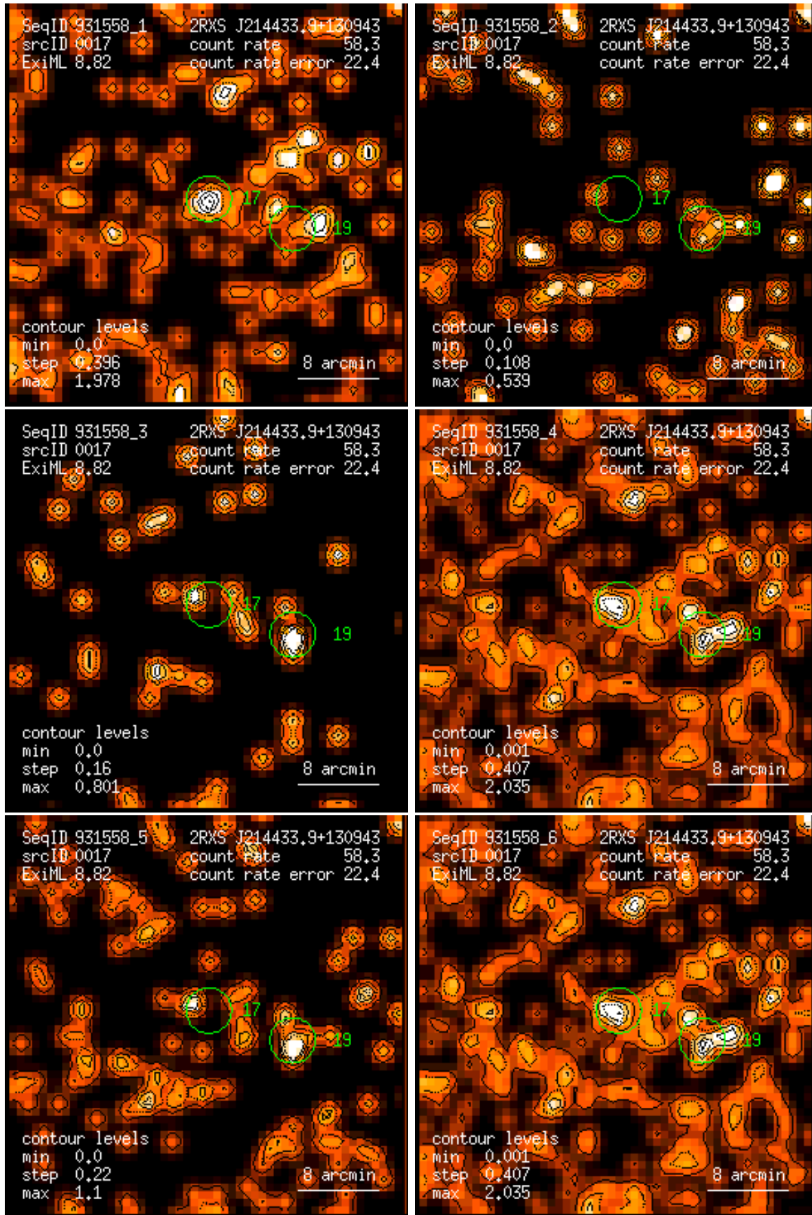
Figure 17: RASS 931558: detection 0017: band rate images, Gaussian filter: (1) PSPC channels 11 – 41, (2) 52 – 90, (3) 91 – 201, (4) 11 – 235, (5) 52 – 201, (6) 11 – 201. Broad band rates in counts/ks. Band rate contour levels in counts/ks/arcmin 2 .
