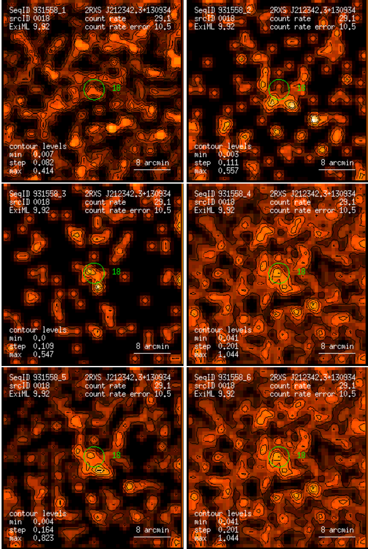
Figure 18: RASS 931558: detection 0018: band rate images, Gaussian filter: (1) PSPC channels 11 – 41, (2) 52 – 90, (3) 91 – 201, (4) 11 – 235, (5) 52 – 201, (6) 11 – 201. Broad band rates in counts/ks. Band rate contour levels in counts/ks/arcmin 2 .
