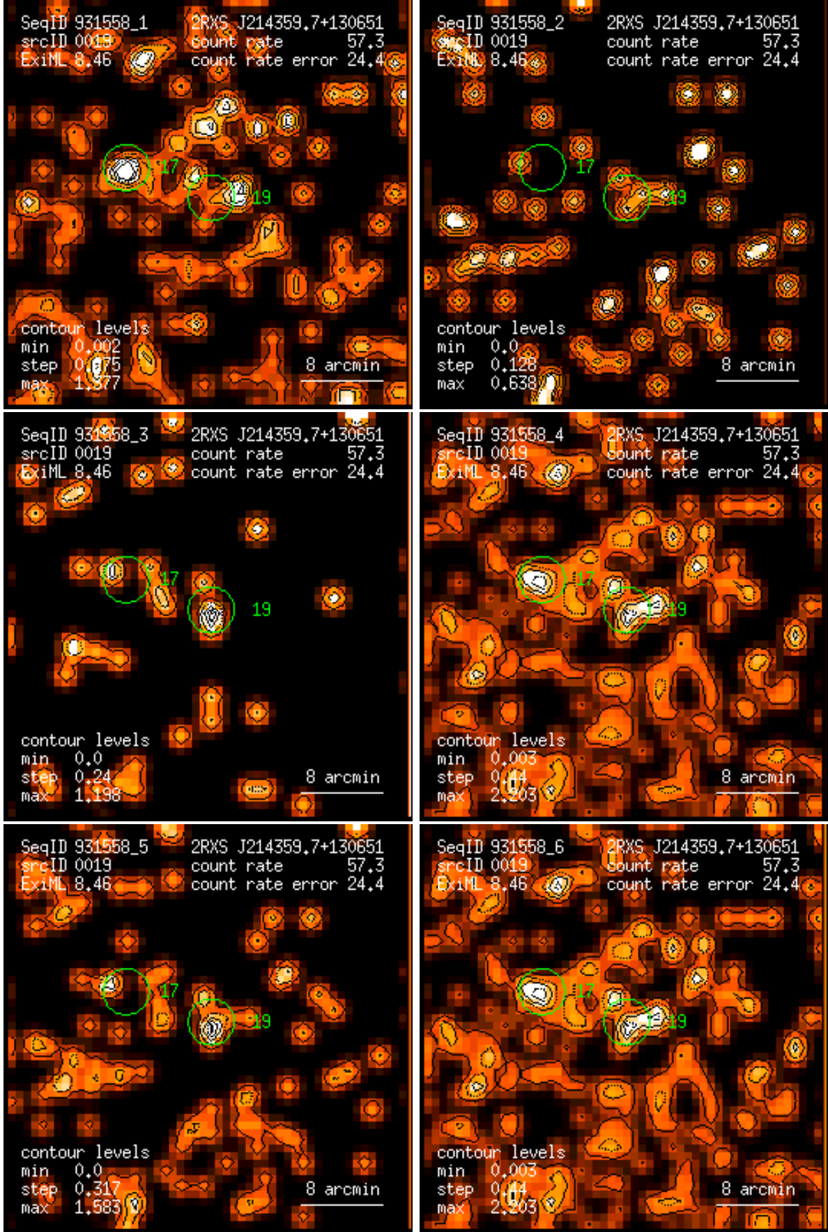
Figure 19: RASS 931558: detection 0019: band rate images, Gaussian filter: (1) PSPC channels 11 – 41, (2) 52 – 90, (3) 91 – 201, (4) 11 – 235, (5) 52 – 201, (6) 11 – 201. Broad band rates in counts/ks. Band rate contour levels in counts/ks/arcmin 2 .
