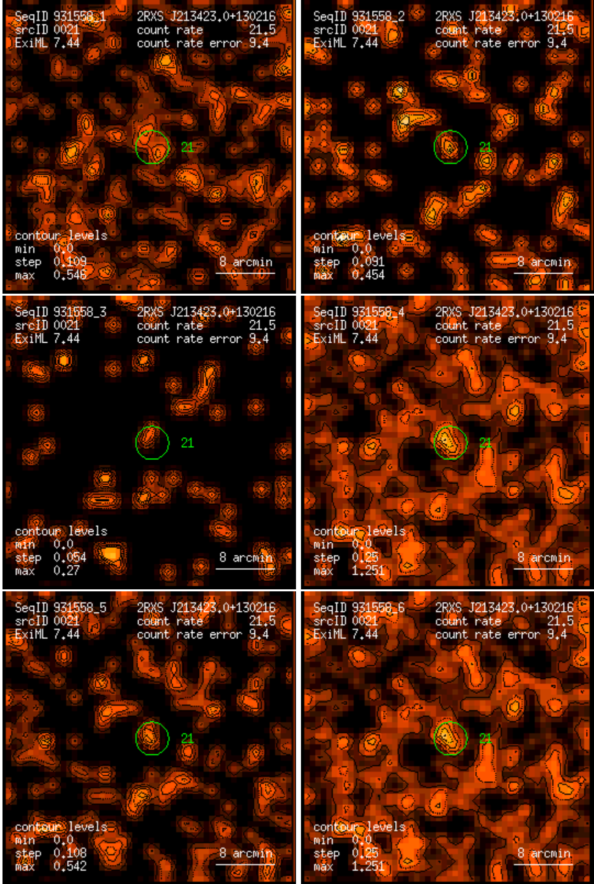
Figure 21: RASS 931558: detection 0021: band rate images, Gaussian filter: (1) PSPC channels 11 – 41, (2) 52 – 90, (3) 91 – 201, (4) 11 – 235, (5) 52 – 201, (6) 11 – 201. Broad band rates in counts/ks. Band rate contour levels in counts/ks/arcmin 2 .
