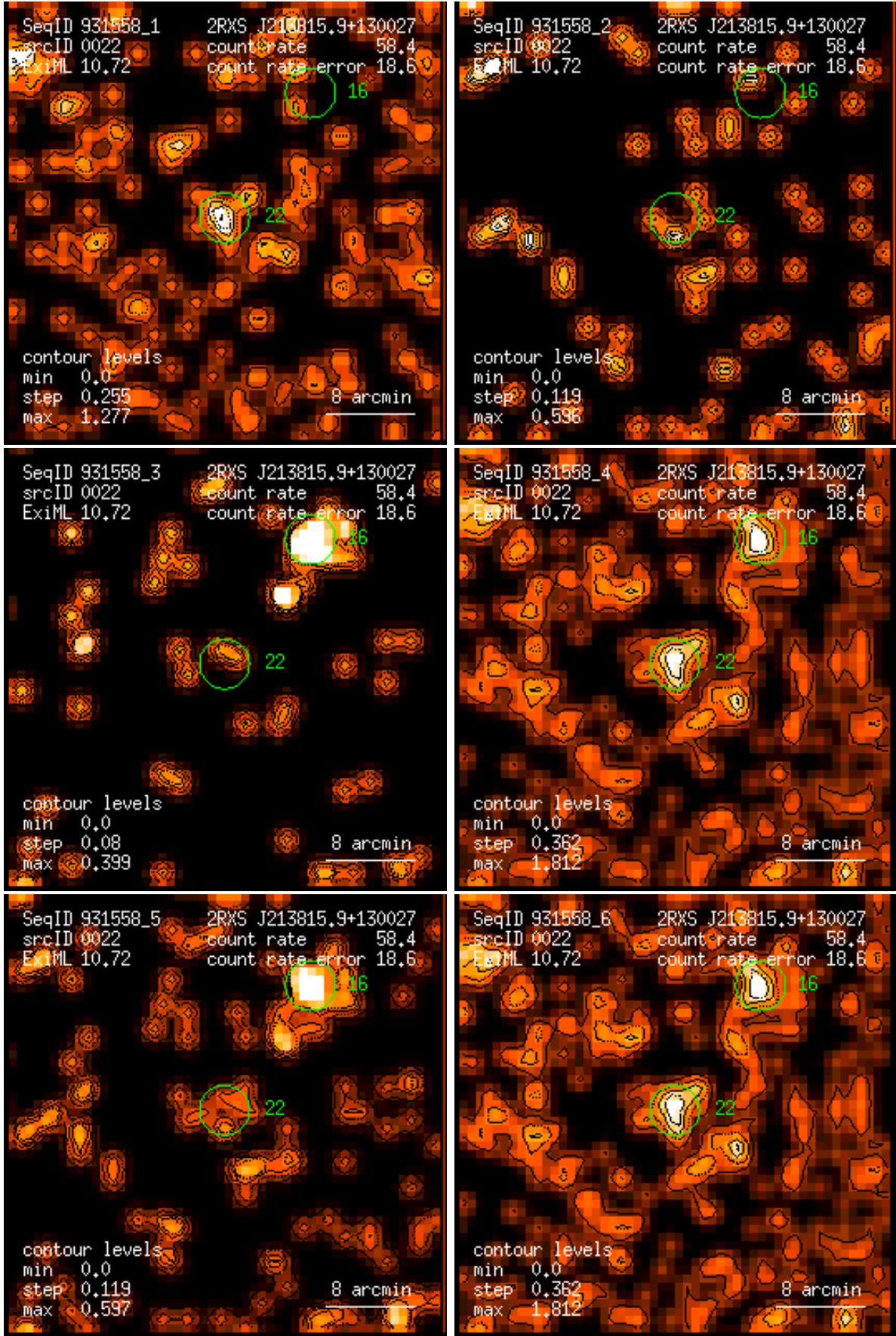
Figure 22: RASS 931558: detection 0022: band rate images, Gaussian filter: (1) PSPC channels 11 – 41, (2) 52 – 90, (3) 91 – 201, (4) 11 – 235, (5) 52 – 201, (6) 11 – 201. Broad band rates in counts/ks. Band rate contour levels in counts/ks/arcmin 2 .
