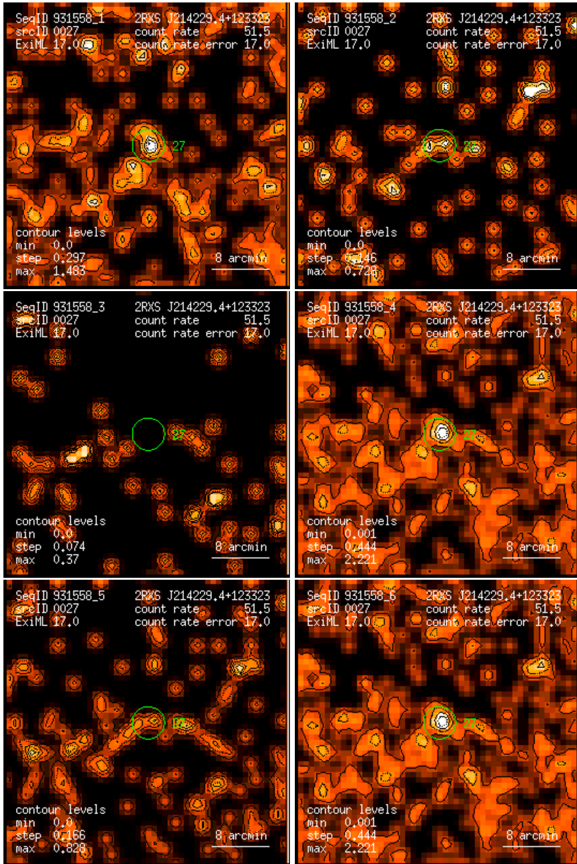
Figure 27: RASS 931558: detection 0027: band rate images, Gaussian filter: (1) PSPC channels 11 – 41, (2) 52 – 90, (3) 91 – 201, (4) 11 – 235, (5) 52 – 201, (6) 11 – 201. Broad band rates in counts/ks. Band rate contour levels in counts/ks/arcmin 2 .
