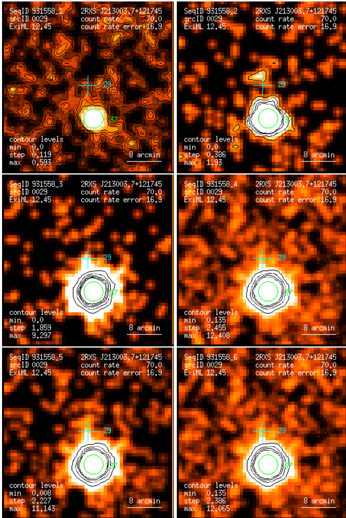
Figure 29: RASS 931558: detection 0029: band rate images, Gaussian filter: (1) PSPC channels 11 – 41, (2) 52 – 90, (3) 91 – 201, (4) 11 – 235, (5) 52 – 201, (6) 11 – 201. Broad band rates in counts/ks. Band rate contour levels in counts/ks/arcmin 2 .
