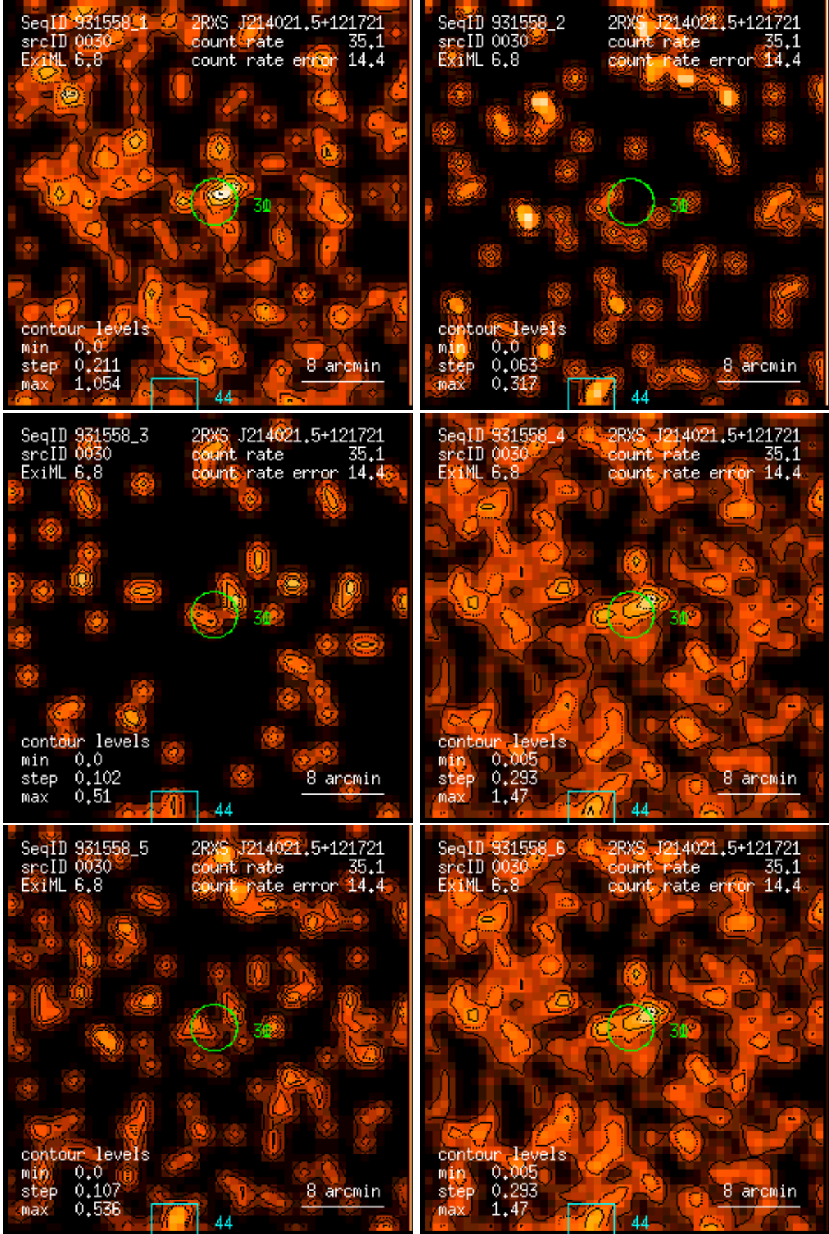
Figure 30: RASS 931558: detection 0030: band rate images, Gaussian filter: (1) PSPC channels 11 – 41, (2) 52 – 90, (3) 91 – 201, (4) 11 – 235, (5) 52 – 201, (6) 11 – 201. Broad band rates in counts/ks. Band rate contour levels in counts/ks/arcmin 2 .
