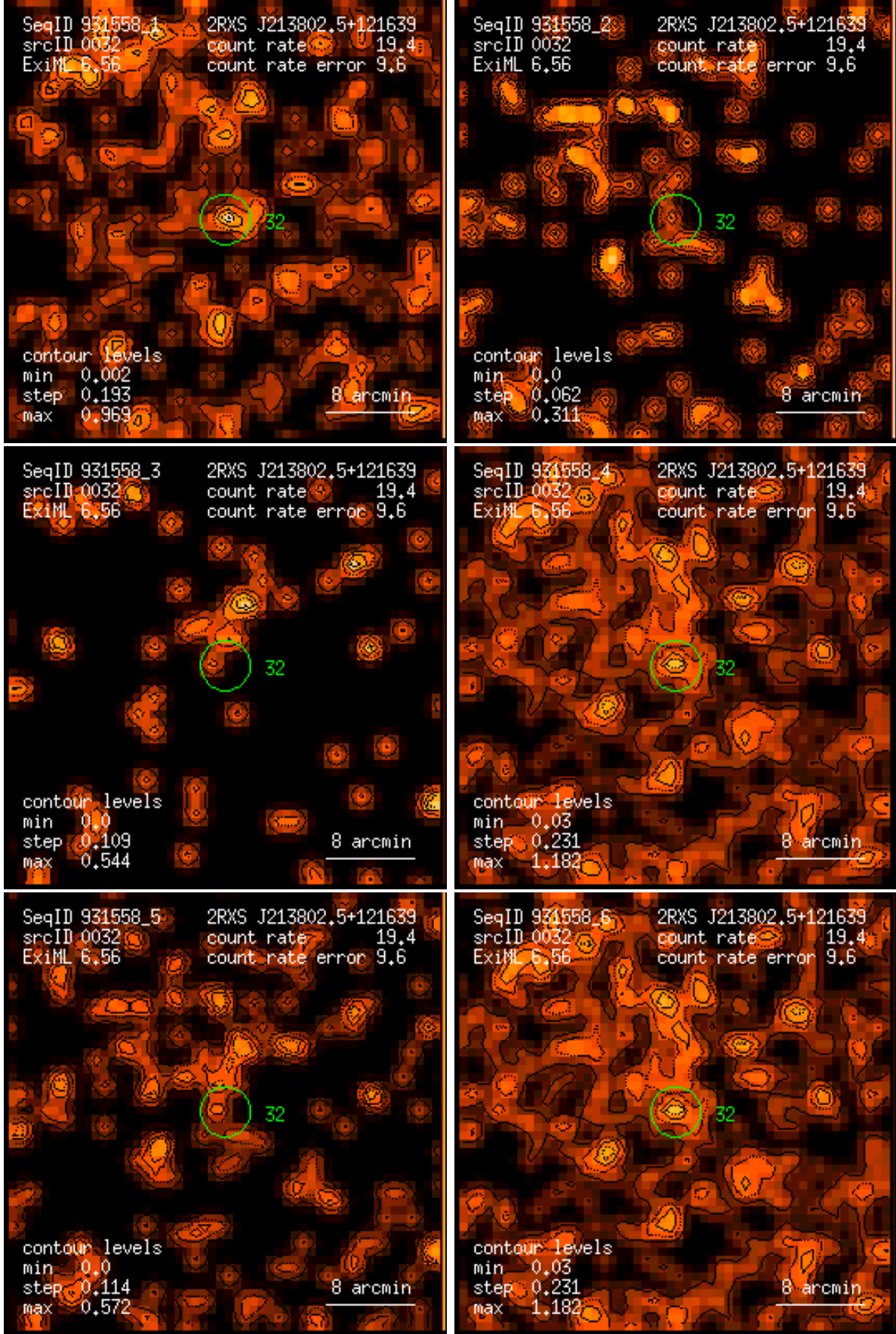
Figure 32: RASS 931558: detection 0032: band rate images, Gaussian filter: (1) PSPC channels 11 – 41, (2) 52 – 90, (3) 91 – 201, (4) 11 – 235, (5) 52 – 201, (6) 11 – 201. Broad band rates in counts/ks. Band rate contour levels in counts/ks/arcmin 2 .
