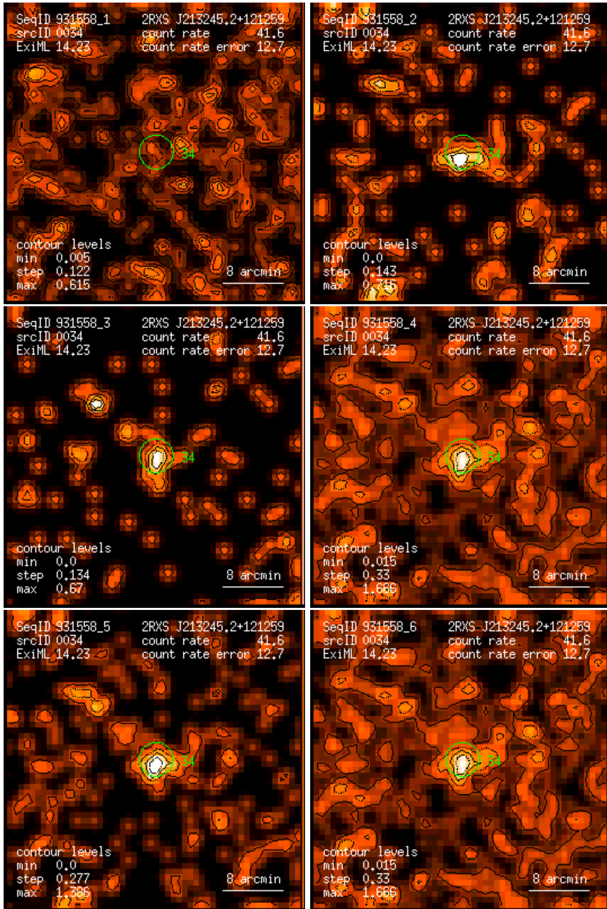
Figure 34: RASS 931558: detection 0034: band rate images, Gaussian filter: (1) PSPC channels 11 – 41, (2) 52 – 90, (3) 91 – 201, (4) 11 – 235, (5) 52 – 201, (6) 11 – 201. Broad band rates in counts/ks. Band rate contour levels in counts/ks/arcmin 2 .
