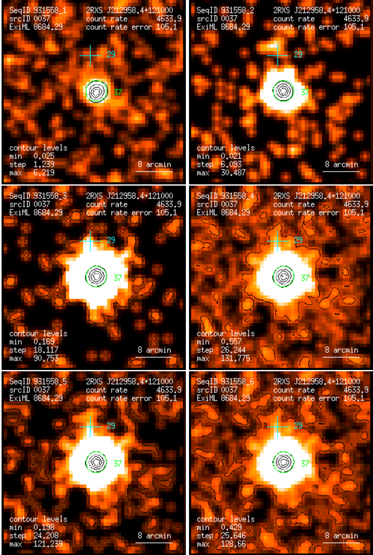
Figure 37: RASS 931558: detection 0037: band rate images, Gaussian filter: (1) PSPC channels 11 – 41, (2) 52 – 90, (3) 91 – 201, (4) 11 – 235, (5) 52 – 201, (6) 11 – 201. Broad band rates in counts/ks. Band rate contour levels in counts/ks/arcmin 2 .
