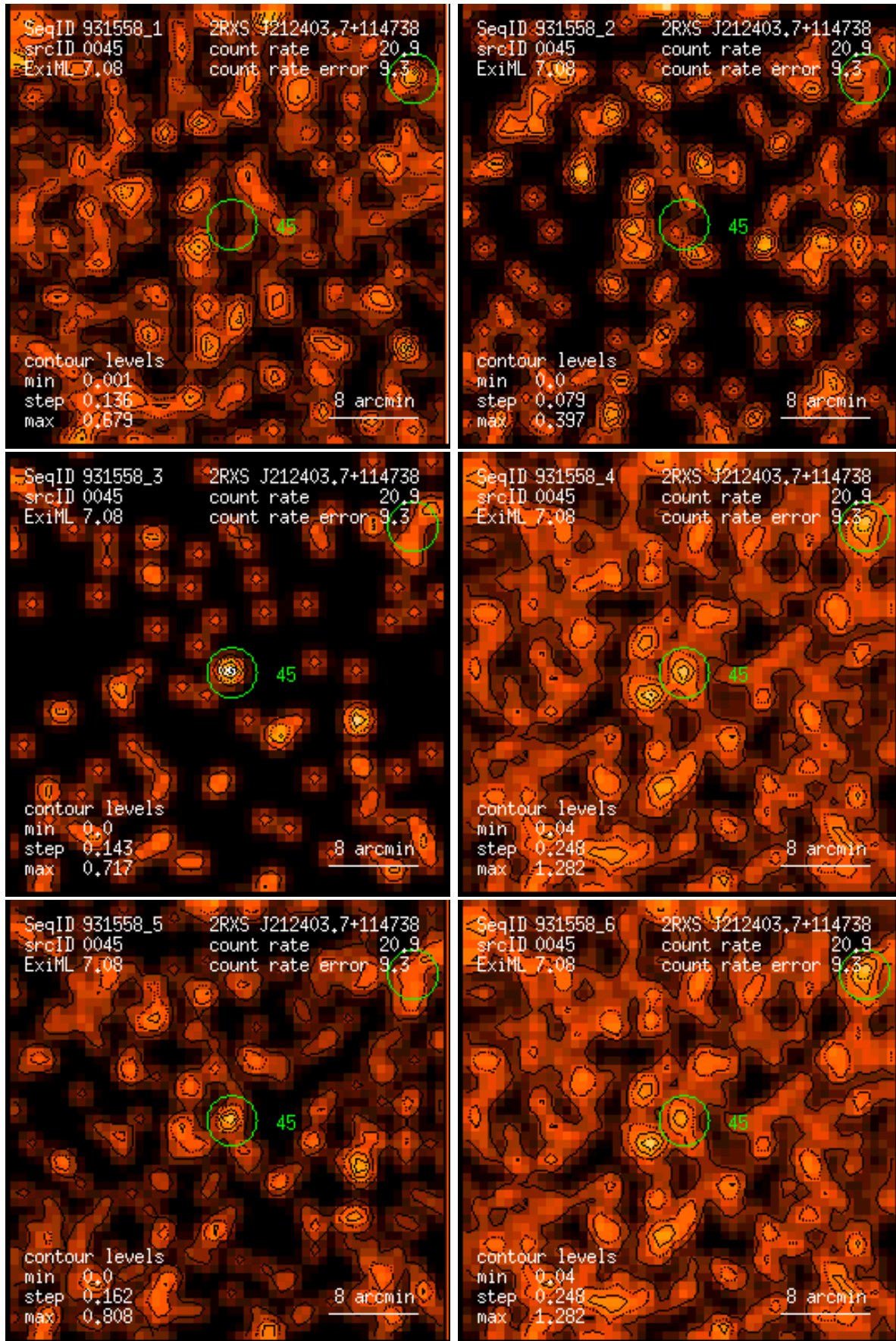
Figure 45: RASS 931558: detection 0045: band rate images, Gaussian filter: (1) PSPC channels 11 – 41, (2) 52 – 90, (3) 91 – 201, (4) 11 – 235, (5) 52 – 201, (6) 11 – 201. Broad band rates in counts/ks. Band rate contour levels in counts/ks/arcmin 2 .
