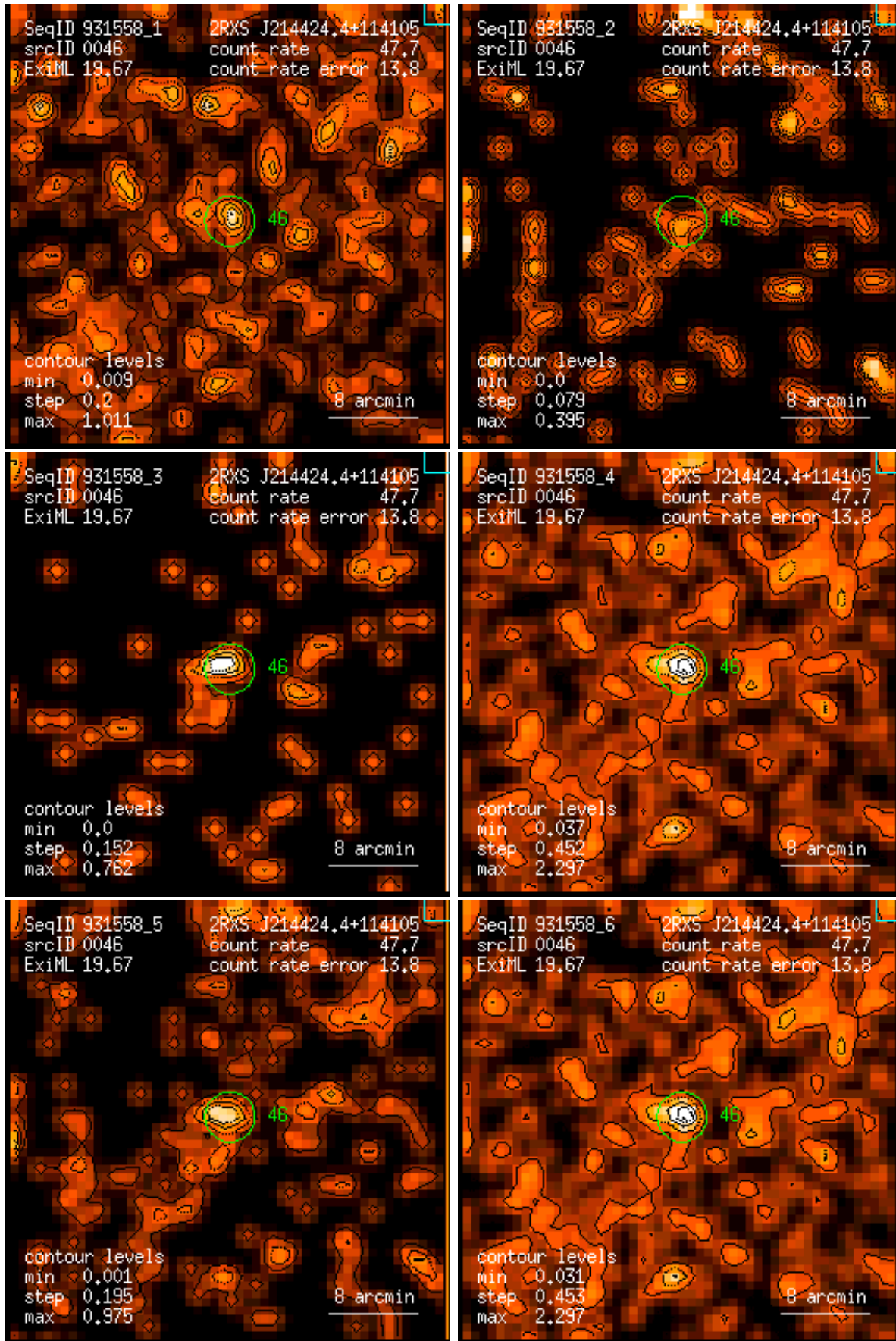
Figure 46: RASS 931558: detection 0046: band rate images, Gaussian filter: (1) PSPC channels 11 – 41, (2) 52 – 90, (3) 91 – 201, (4) 11 – 235, (5) 52 – 201, (6) 11 – 201. Broad band rates in counts/ks. Band rate contour levels in counts/ks/arcmin 2 .
