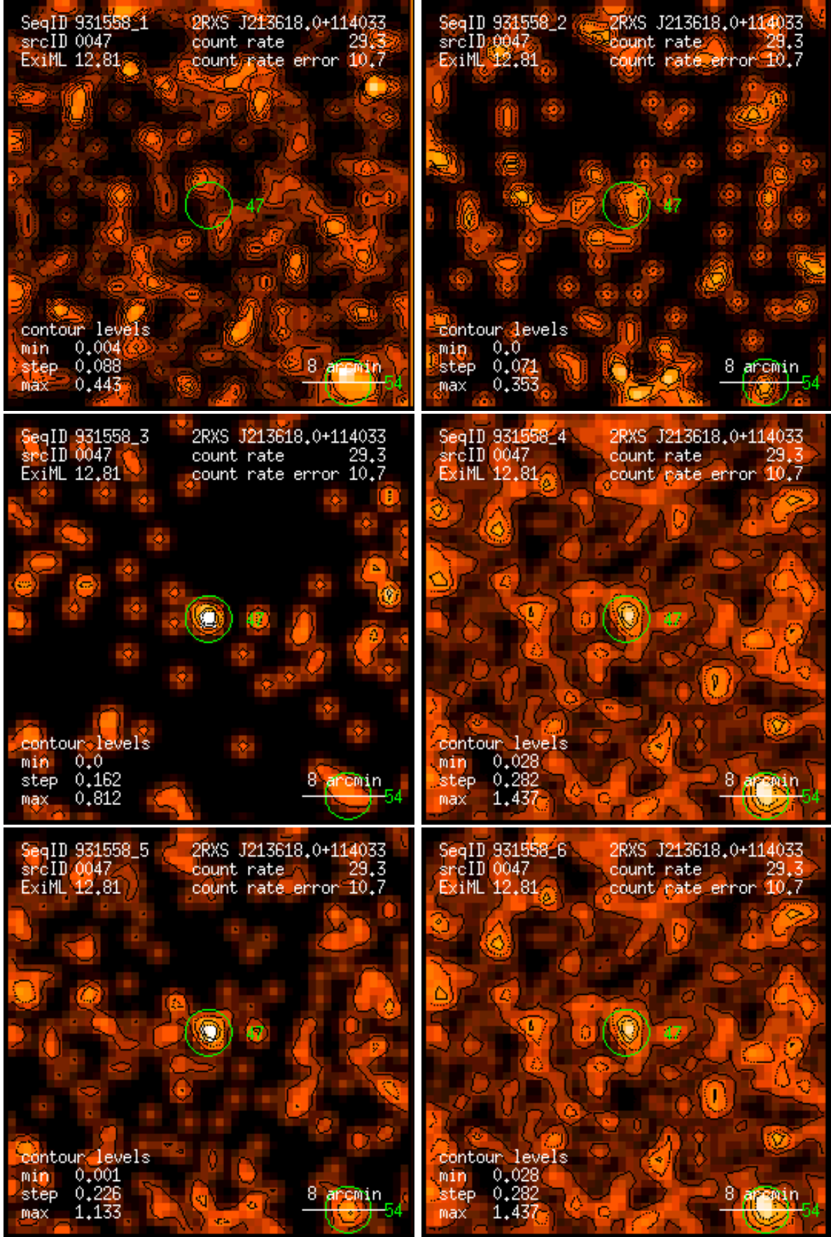
Figure 47: RASS 931558: detection 0047: band rate images, Gaussian filter: (1) PSPC channels 11 – 41, (2) 52 – 90, (3) 91 – 201, (4) 11 – 235, (5) 52 – 201, (6) 11 – 201. Broad band rates in counts/ks. Band rate contour levels in counts/ks/arcmin 2 .
