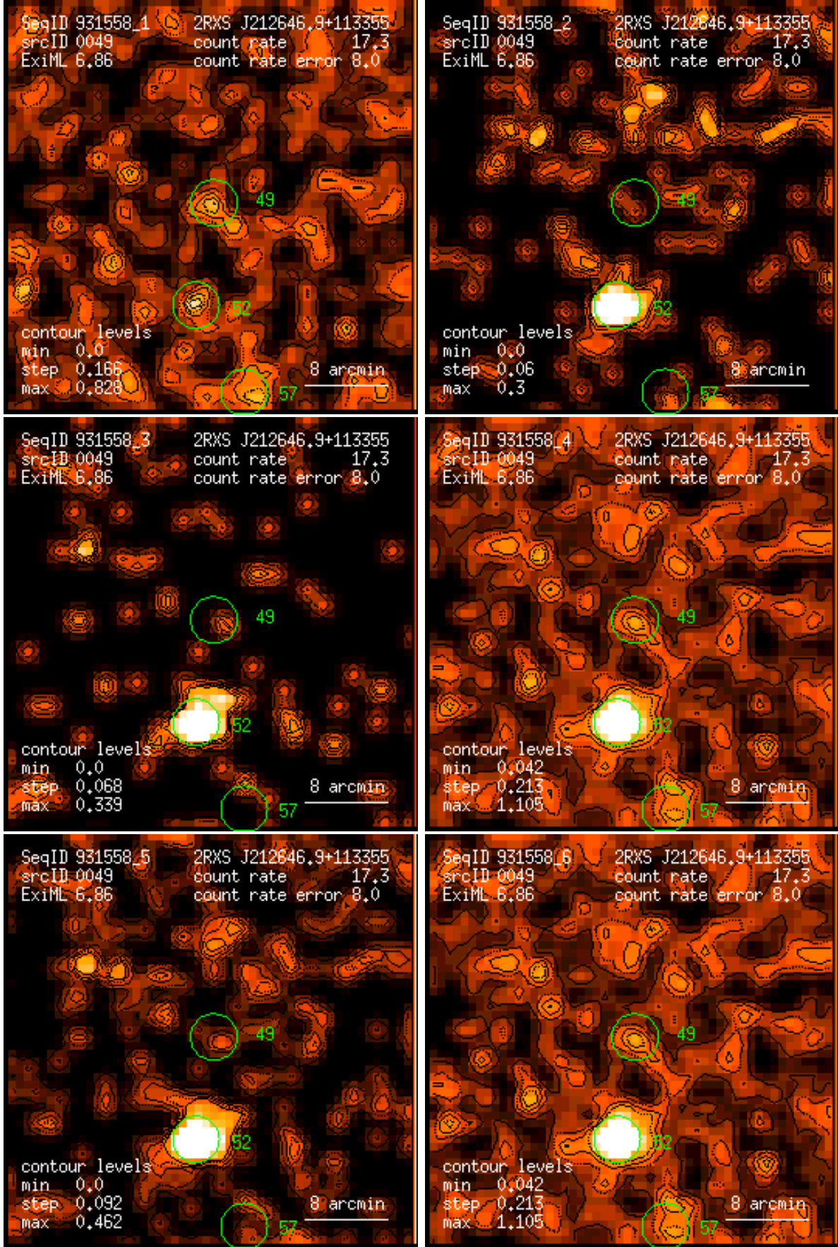
Figure 49: RASS 931558: detection 0049: band rate images, Gaussian filter: (1) PSPC channels 11 – 41, (2) 52 – 90, (3) 91 – 201, (4) 11 – 235, (5) 52 – 201, (6) 11 – 201. Broad band rates in counts/ks. Band rate contour levels in counts/ks/arcmin 2 .
