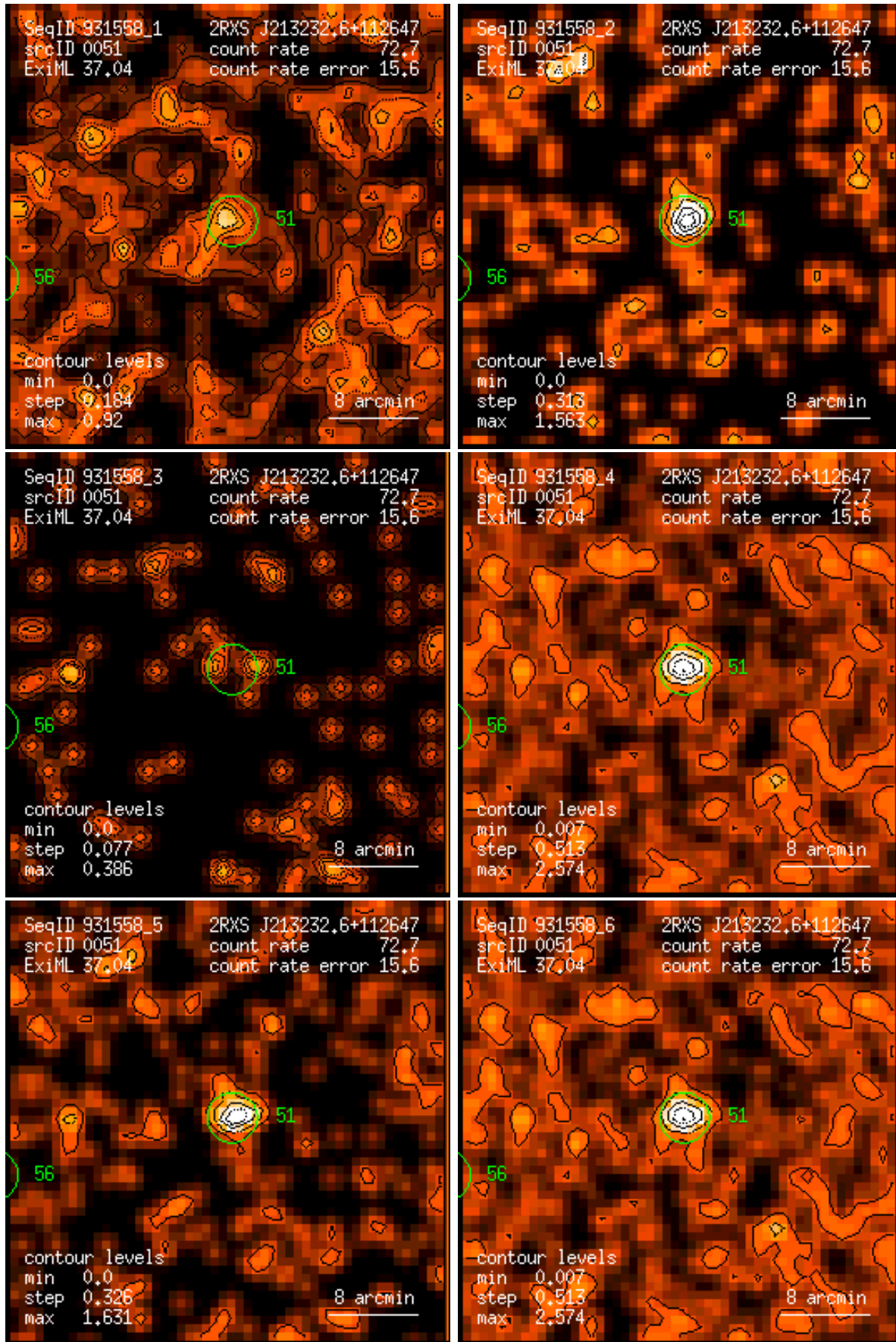
Figure 51: RASS 931558: detection 0051: band rate images, Gaussian filter: (1) PSPC channels 11 – 41, (2) 52 – 90, (3) 91 – 201, (4) 11 – 235, (5) 52 – 201, (6) 11 – 201. Broad band rates in counts/ks. Band rate contour levels in counts/ks/arcmin 2 .
