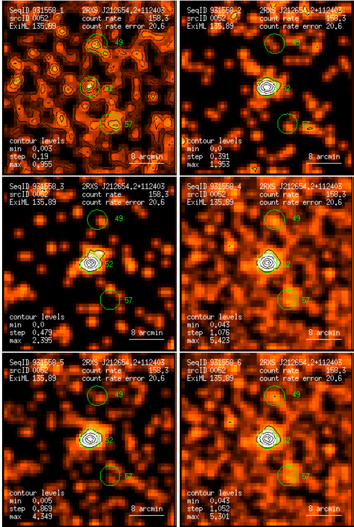
Figure 52: RASS 931558: detection 0052: band rate images, Gaussian filter: (1) PSPC channels 11 – 41, (2) 52 – 90, (3) 91 – 201, (4) 11 – 235, (5) 52 – 201, (6) 11 – 201. Broad band rates in counts/ks. Band rate contour levels in counts/ks/arcmin 2 .
