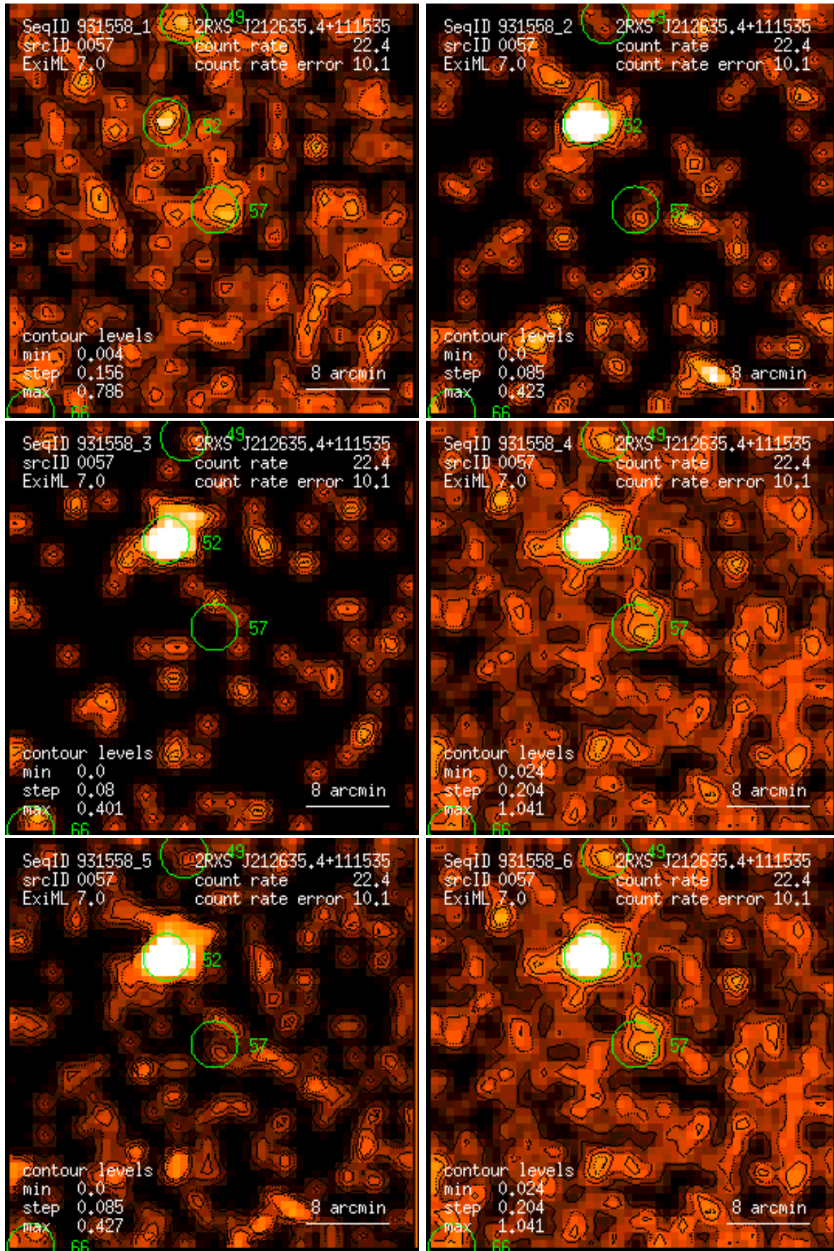
Figure 57: RASS 931558: detection 0057: band rate images, Gaussian filter: (1) PSPC channels 11 – 41, (2) 52 – 90, (3) 91 – 201, (4) 11 – 235, (5) 52 – 201, (6) 11 – 201. Broad band rates in counts/ks. Band rate contour levels in counts/ks/arcmin 2 .
