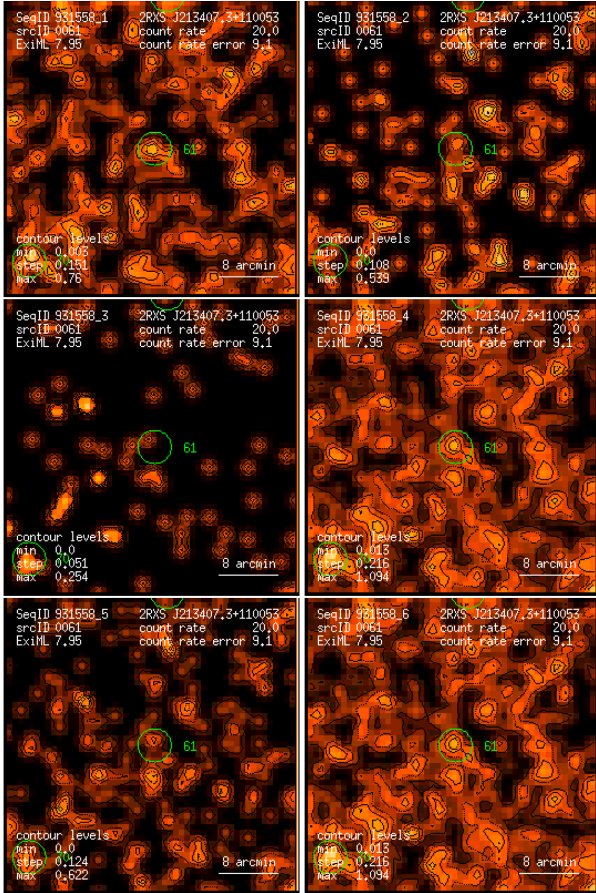
Figure 61: RASS 931558: detection 0061: band rate images, Gaussian filter: (1) PSPC channels 11 – 41, (2) 52 – 90, (3) 91 – 201, (4) 11 – 235, (5) 52 – 201, (6) 11 – 201. Broad band rates in counts/ks. Band rate contour levels in counts/ks/arcmin 2 .
