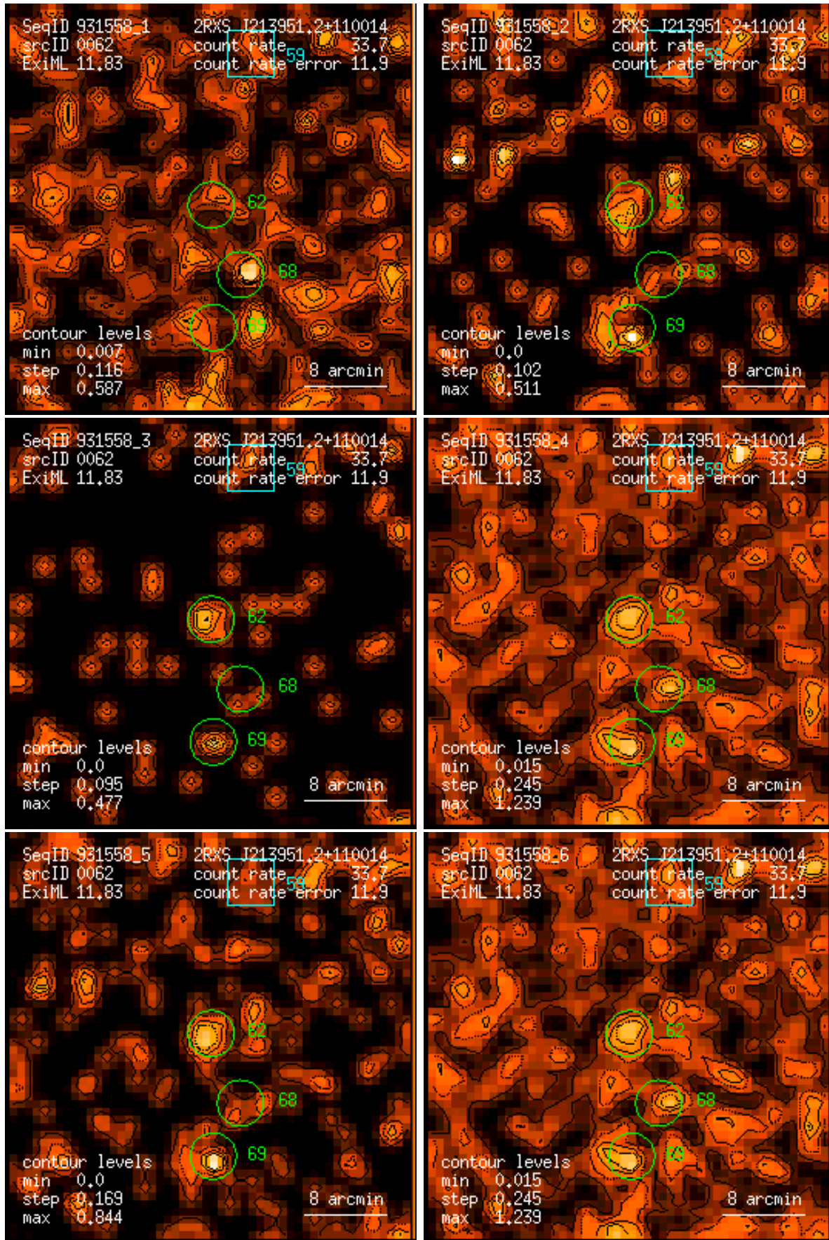
Figure 62: RASS 931558: detection 0062: band rate images, Gaussian filter: (1) PSPC channels 11 – 41, (2) 52 – 90, (3) 91 – 201, (4) 11 – 235, (5) 52 – 201, (6) 11 – 201. Broad band rates in counts/ks. Band rate contour levels in counts/ks/arcmin 2 .
