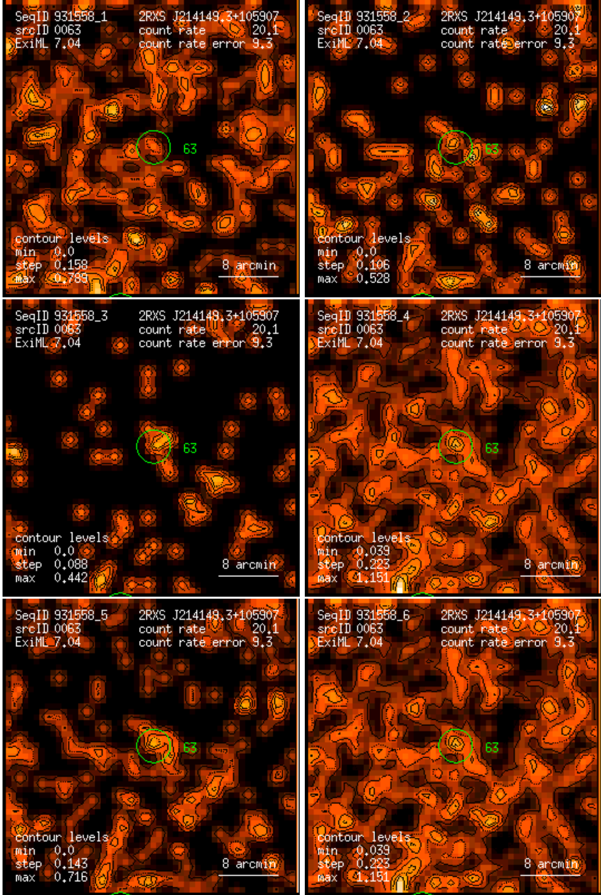
Figure 63: RASS 931558: detection 0063: band rate images, Gaussian filter: (1) PSPC channels 11 – 41, (2) 52 – 90, (3) 91 – 201, (4) 11 – 235, (5) 52 – 201, (6) 11 – 201. Broad band rates in counts/ks. Band rate contour levels in counts/ks/arcmin 2 .
