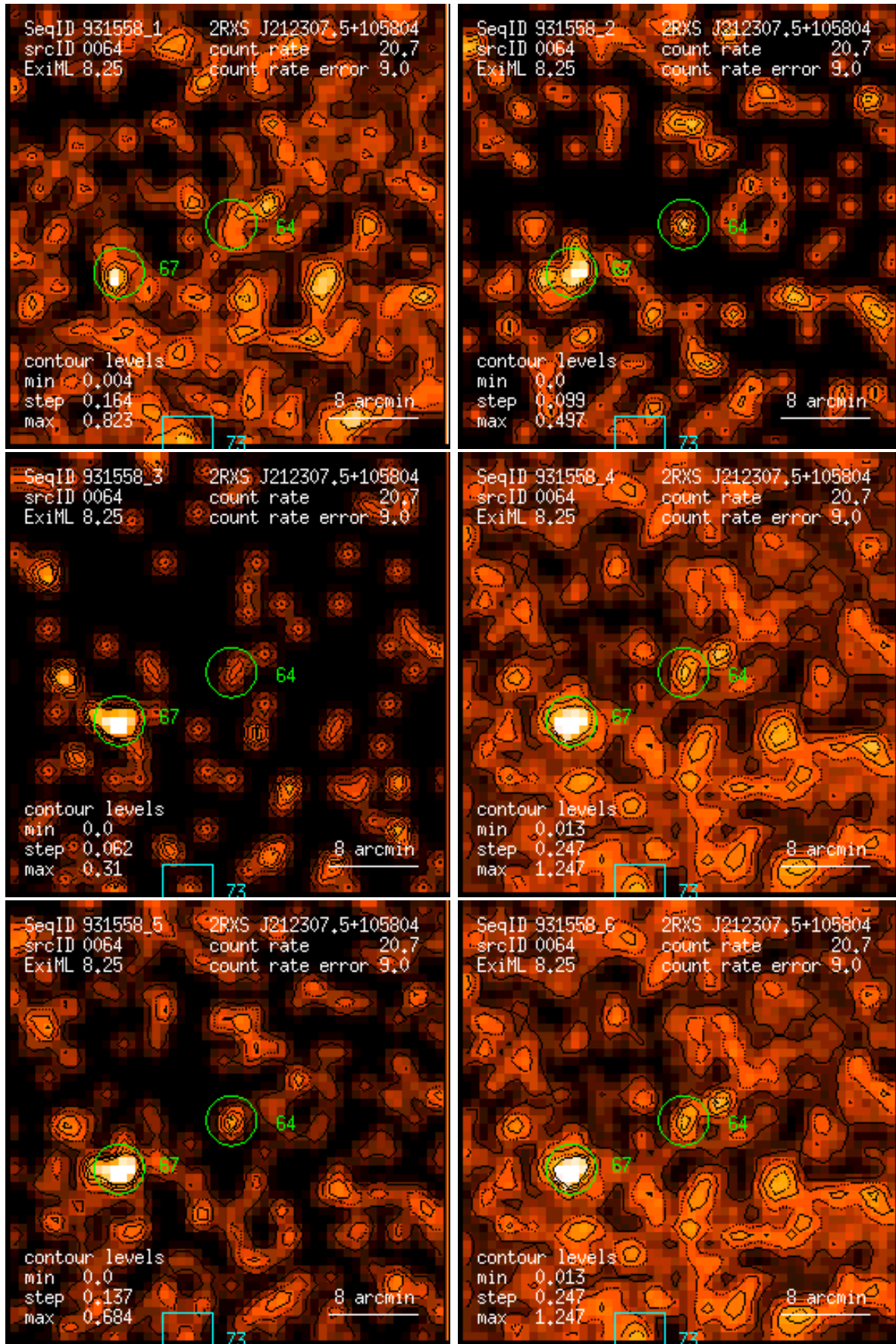
Figure 64: RASS 931558: detection 0064: band rate images, Gaussian filter: (1) PSPC channels 11 – 41, (2) 52 – 90, (3) 91 – 201, (4) 11 – 235, (5) 52 – 201, (6) 11 – 201. Broad band rates in counts/ks. Band rate contour levels in counts/ks/arcmin 2 .
