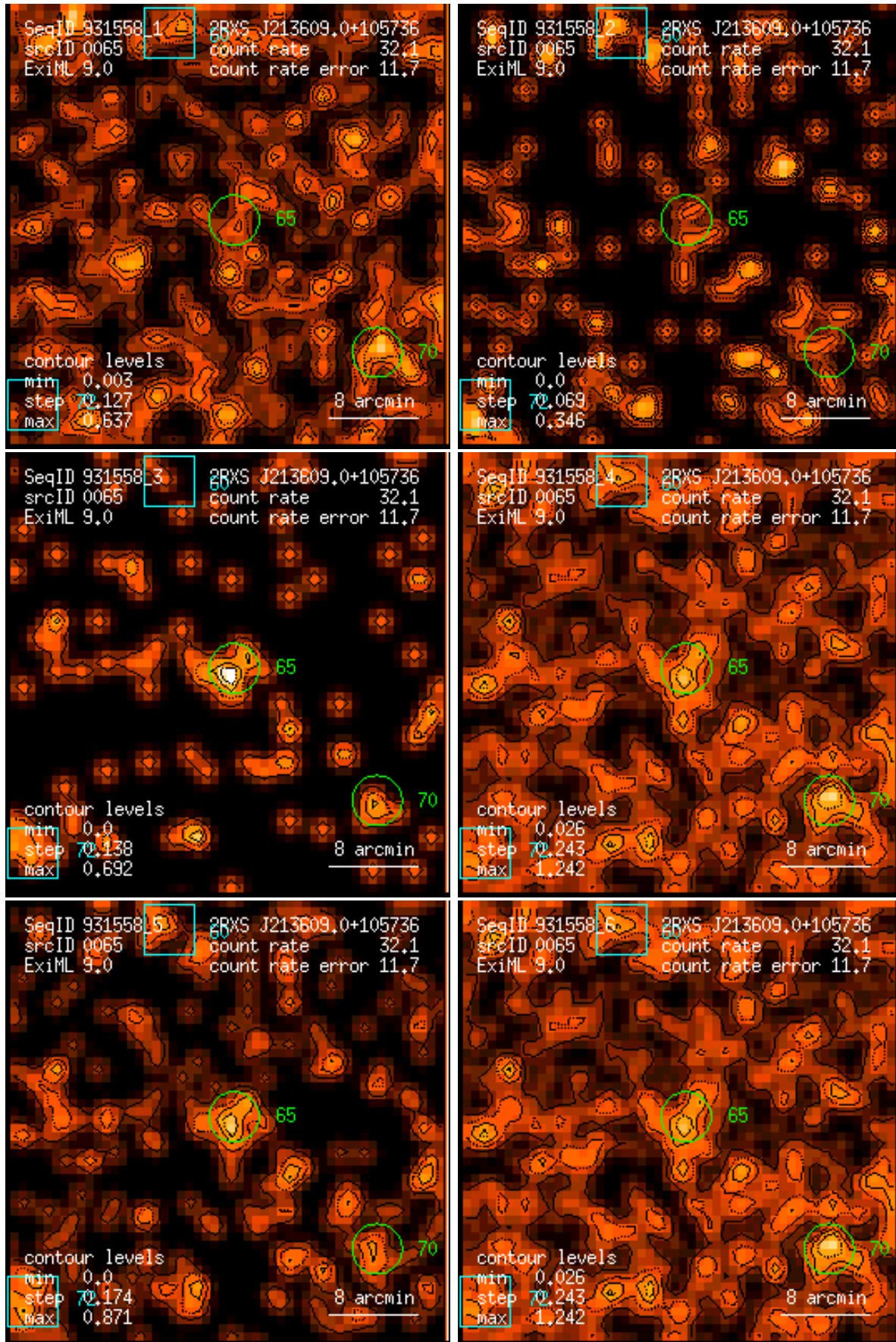
Figure 65: RASS 931558: detection 0065: band rate images, Gaussian filter: (1) PSPC channels 11 – 41, (2) 52 – 90, (3) 91 – 201, (4) 11 – 235, (5) 52 – 201, (6) 11 – 201. Broad band rates in counts/ks. Band rate contour levels in counts/ks/arcmin 2 .
