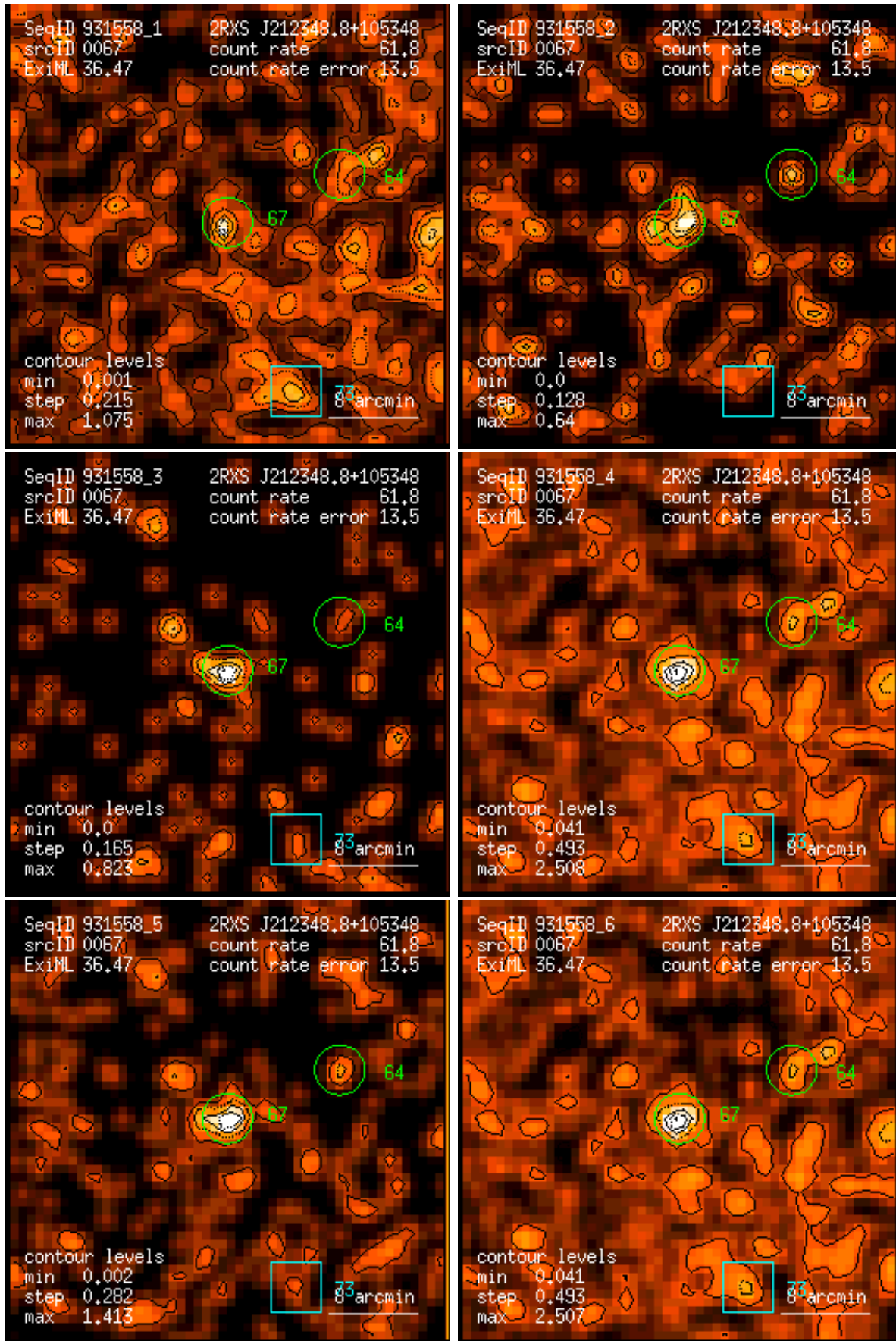
Figure 67: RASS 931558: detection 0067: band rate images, Gaussian filter: (1) PSPC channels 11 – 41, (2) 52 – 90, (3) 91 – 201, (4) 11 – 235, (5) 52 – 201, (6) 11 – 201. Broad band rates in counts/ks. Band rate contour levels in counts/ks/arcmin 2 .
