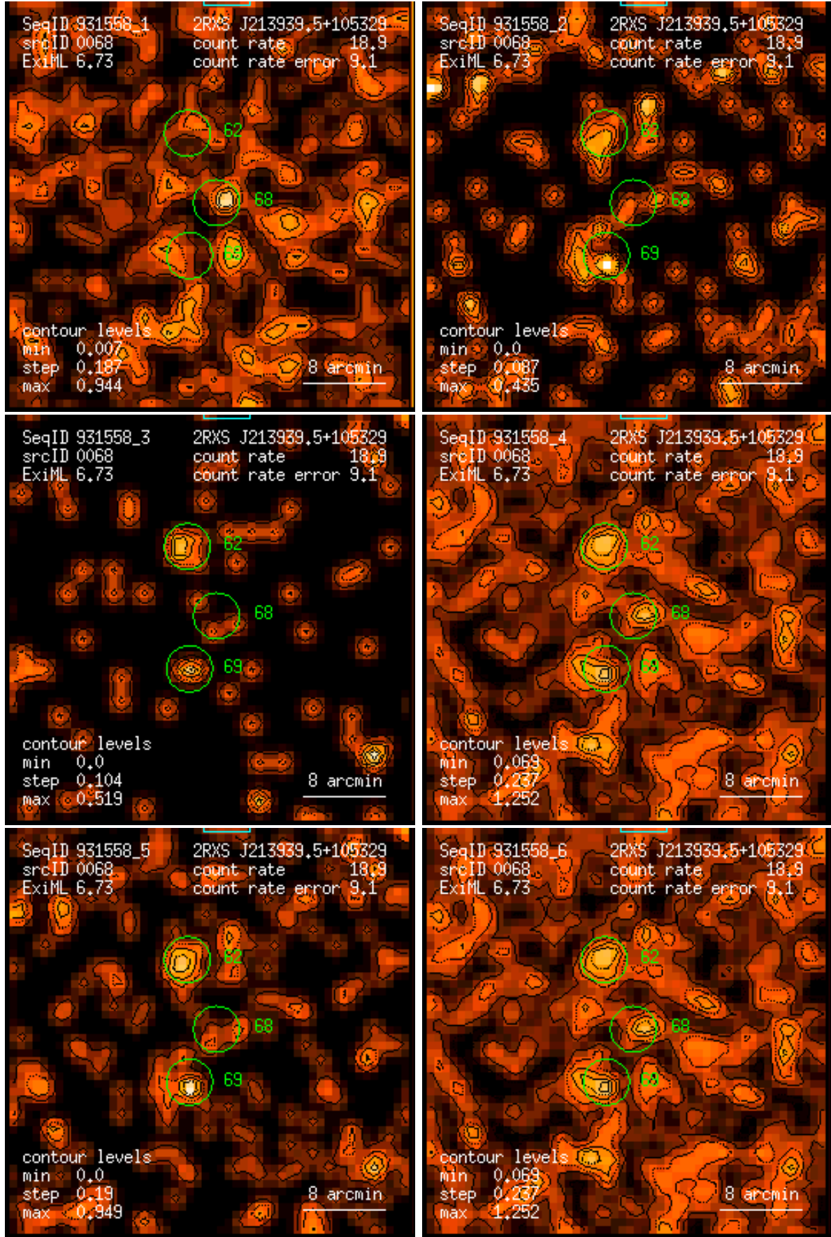
Figure 68: RASS 931558: detection 0068: band rate images, Gaussian filter: (1) PSPC channels 11 – 41, (2) 52 – 90, (3) 91 – 201, (4) 11 – 235, (5) 52 – 201, (6) 11 – 201. Broad band rates in counts/ks. Band rate contour levels in counts/ks/arcmin 2 .
