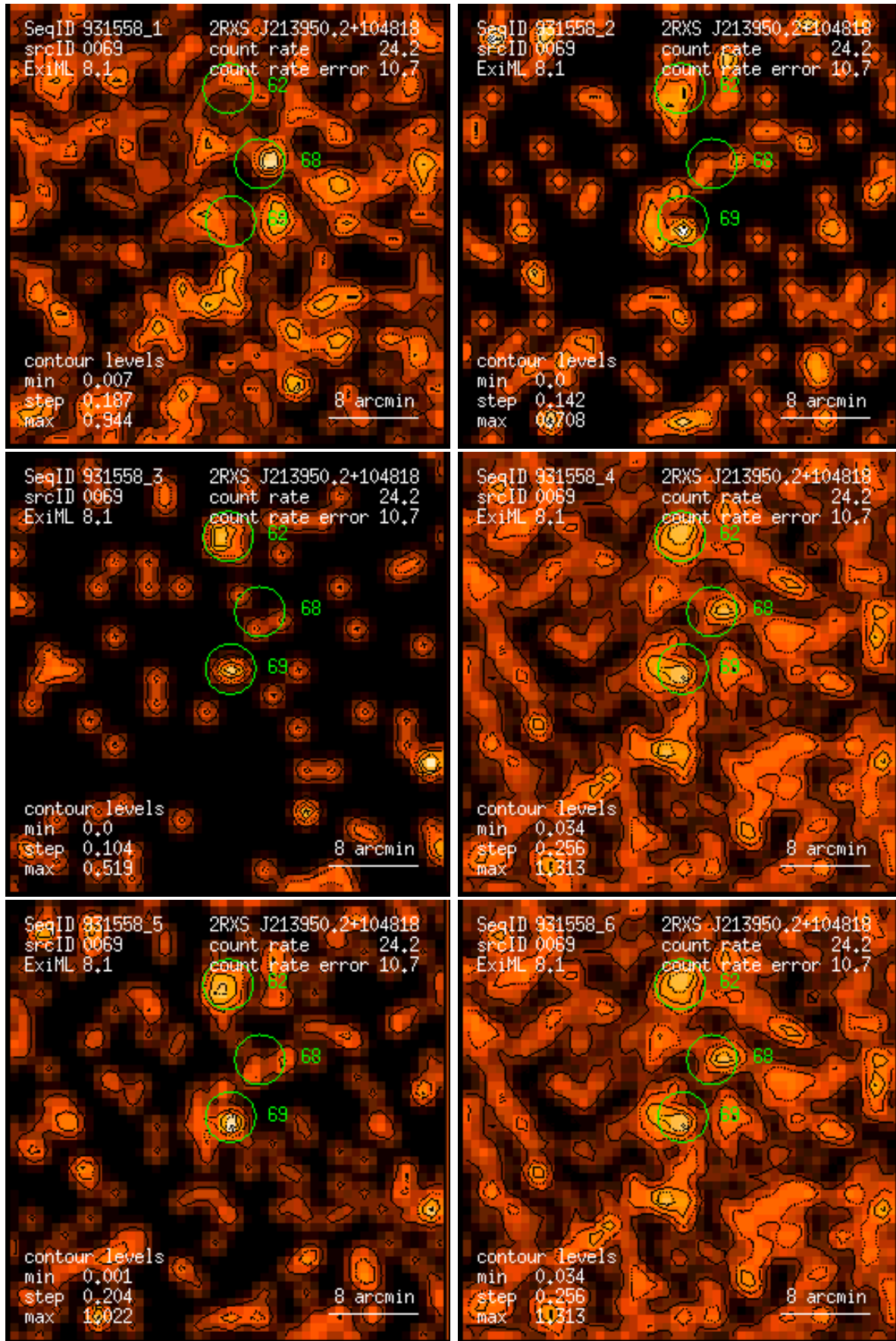
Figure 69: RASS 931558: detection 0069: band rate images, Gaussian filter: (1) PSPC channels 11 – 41, (2) 52 – 90, (3) 91 – 201, (4) 11 – 235, (5) 52 – 201, (6) 11 – 201. Broad band rates in counts/ks. Band rate contour levels in counts/ks/arcmin 2 .
