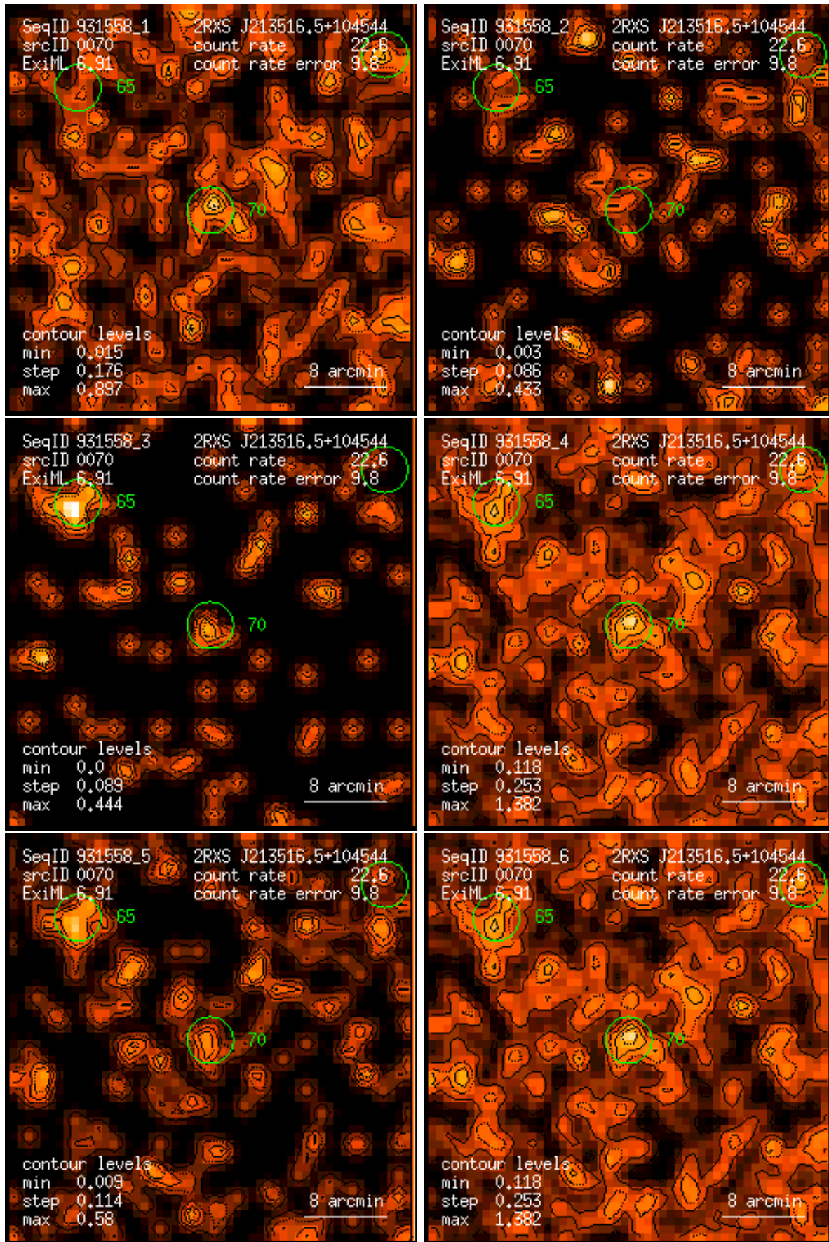
Figure 70: RASS 931558: detection 0070: band rate images, Gaussian filter: (1) PSPC channels 11 – 41, (2) 52 – 90, (3) 91 – 201, (4) 11 – 235, (5) 52 – 201, (6) 11 – 201. Broad band rates in counts/ks. Band rate contour levels in counts/ks/arcmin 2 .
