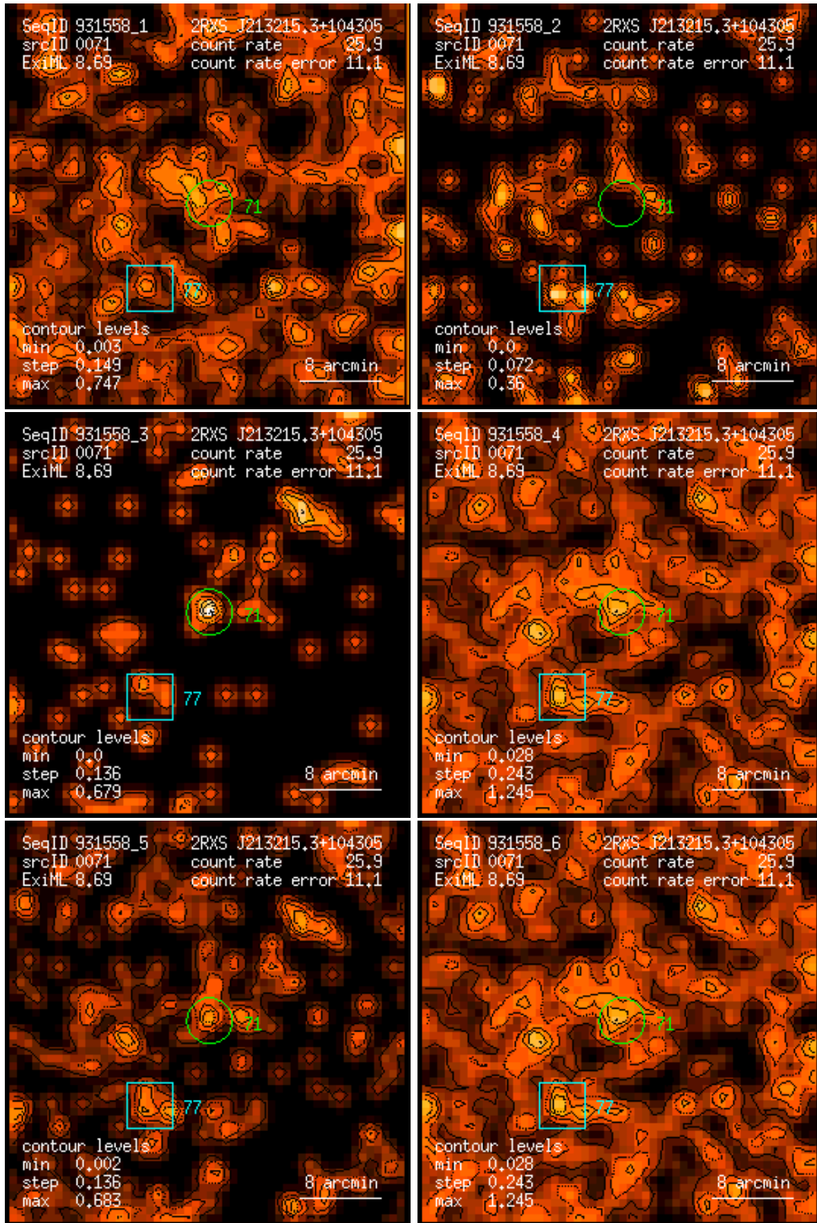
Figure 71: RASS 931558: detection 0071: band rate images, Gaussian filter: (1) PSPP channels 11 – 41, (2) 52 – 90, (3) 91 – 201, (4) 11 – 235, (5) 52 – 201, (6) 11 – 201. Broad band rates in counts/ks. Band rate contour levels in counts/ks/arcmin 2 .
