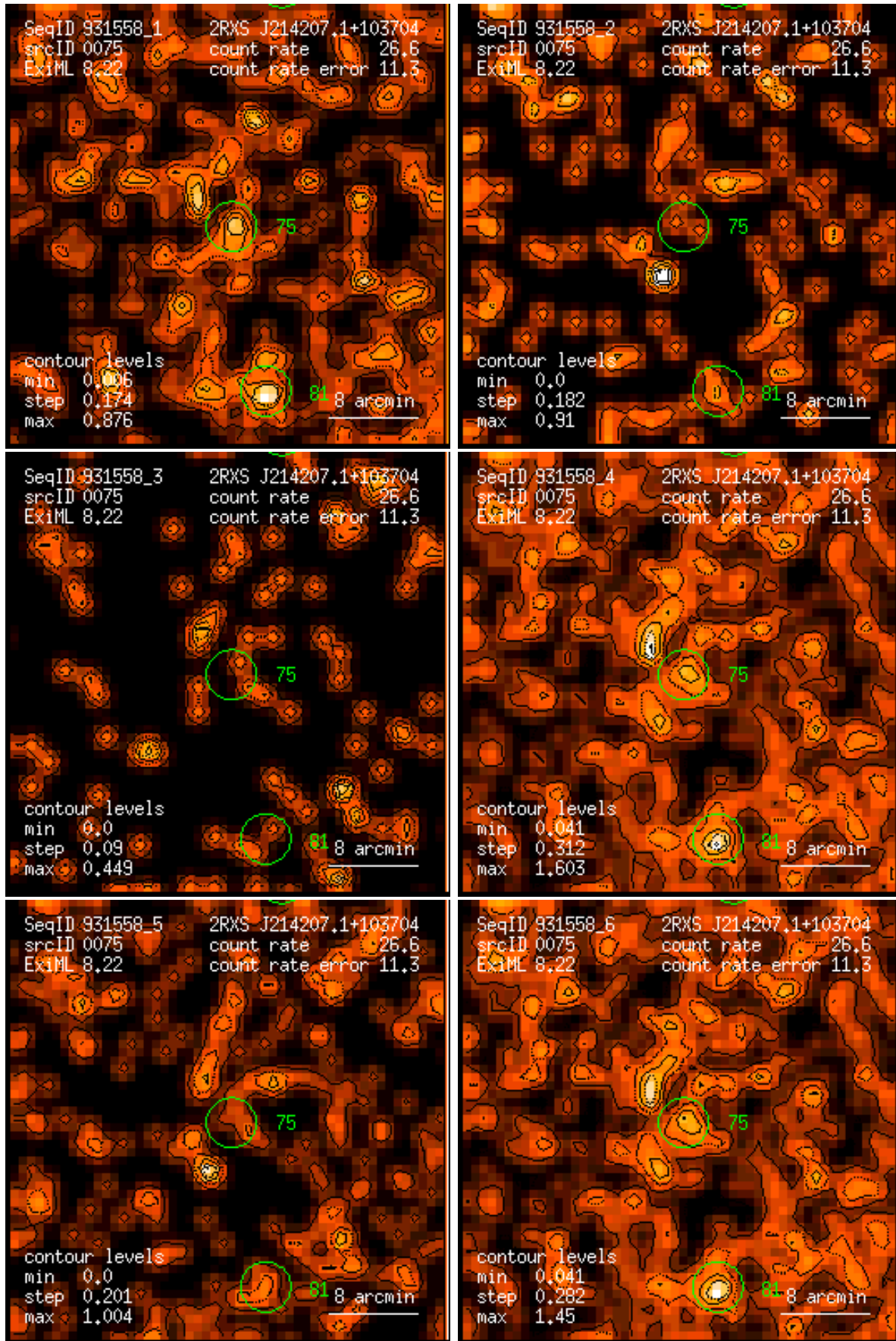
Figure 75: RASS 931558: detection 0075: band rate images, Gaussian filter: (1) PSPC channels 11 – 41, (2) 52 – 90, (3) 91 – 201, (4) 11 – 235, (5) 52 – 201, (6) 11 – 201. Broad band rates in counts/ks. Band rate contour levels in counts/ks/arcmin 2 .
