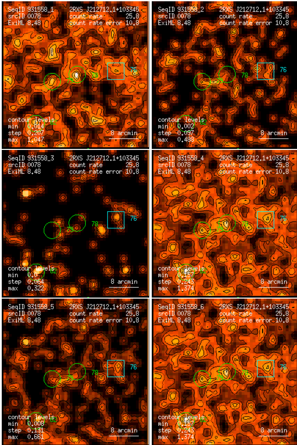
Figure 78: RASS 931558: detection 0078: band rate images, Gaussian filter: (1) PSPC channels 11 – 41, (2) 52 – 90, (3) 91 – 201, (4) 11 – 235, (5) 52 – 201, (6) 11 – 201. Broad band rates in counts/ks. Band rate contour levels in counts/ks/arcmin 2 .
