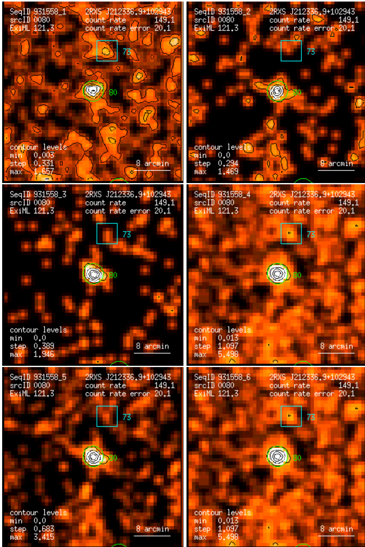
Figure 80: RASS 931558: detection 0080: band rate images, Gaussian filter: (1) PSPC channels 11 – 41, (2) 52 – 90, (3) 91 – 201, (4) 11 – 235, (5) 52 – 201, (6) 11 – 201. Broad band rates in counts/ks. Band rate contour levels in counts/ks/arcmin 2 .
