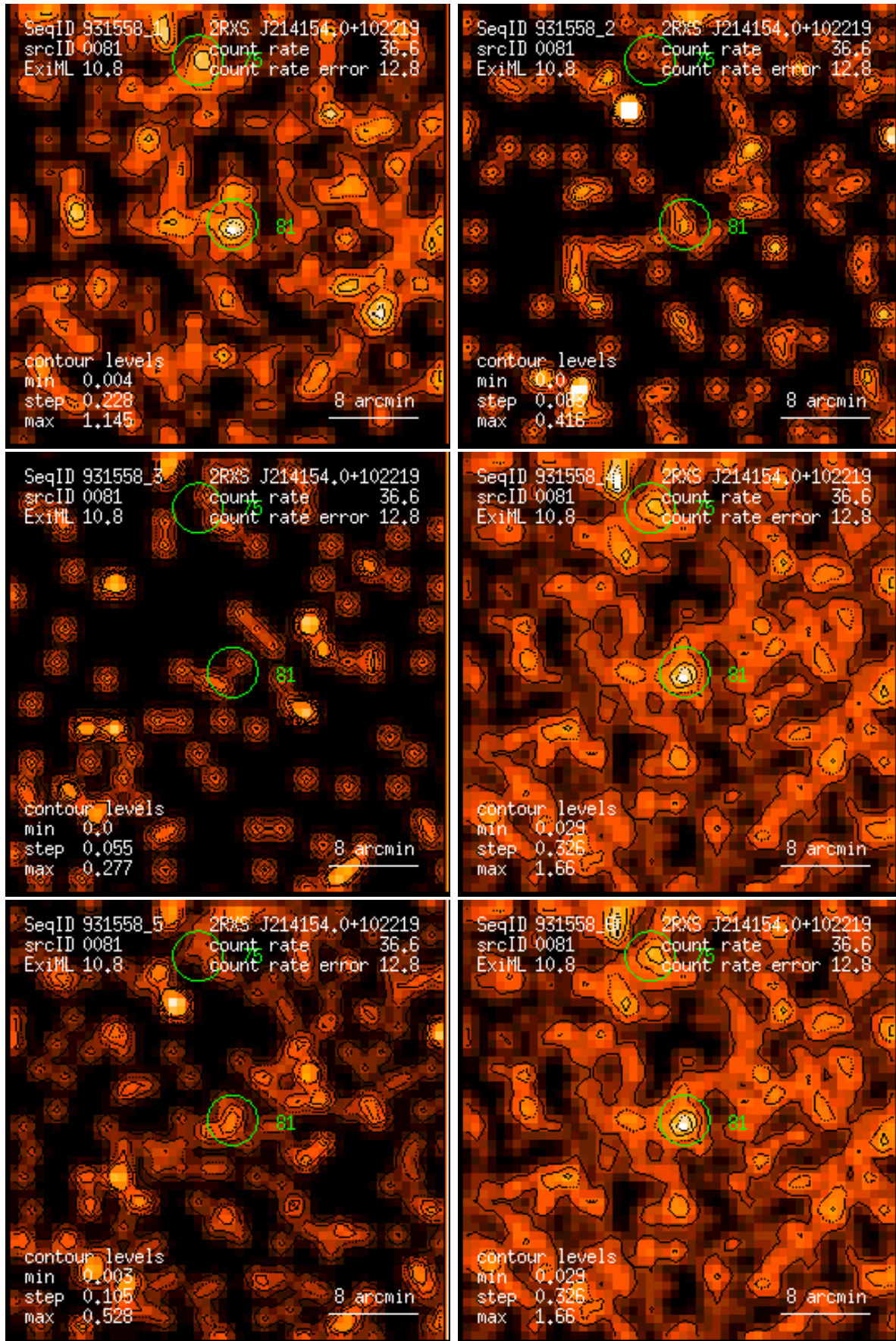
Figure 81: RASS 931558: detection 0081: band rate images, Gaussian filter: (1) PSPC channels 11 – 41, (2) 52 – 90, (3) 91 – 201, (4) 11 – 235, (5) 52 – 201, (6) 11 – 201. Broad band rates in counts/ks. Band rate contour levels in counts/ks/arcmin 2 .
