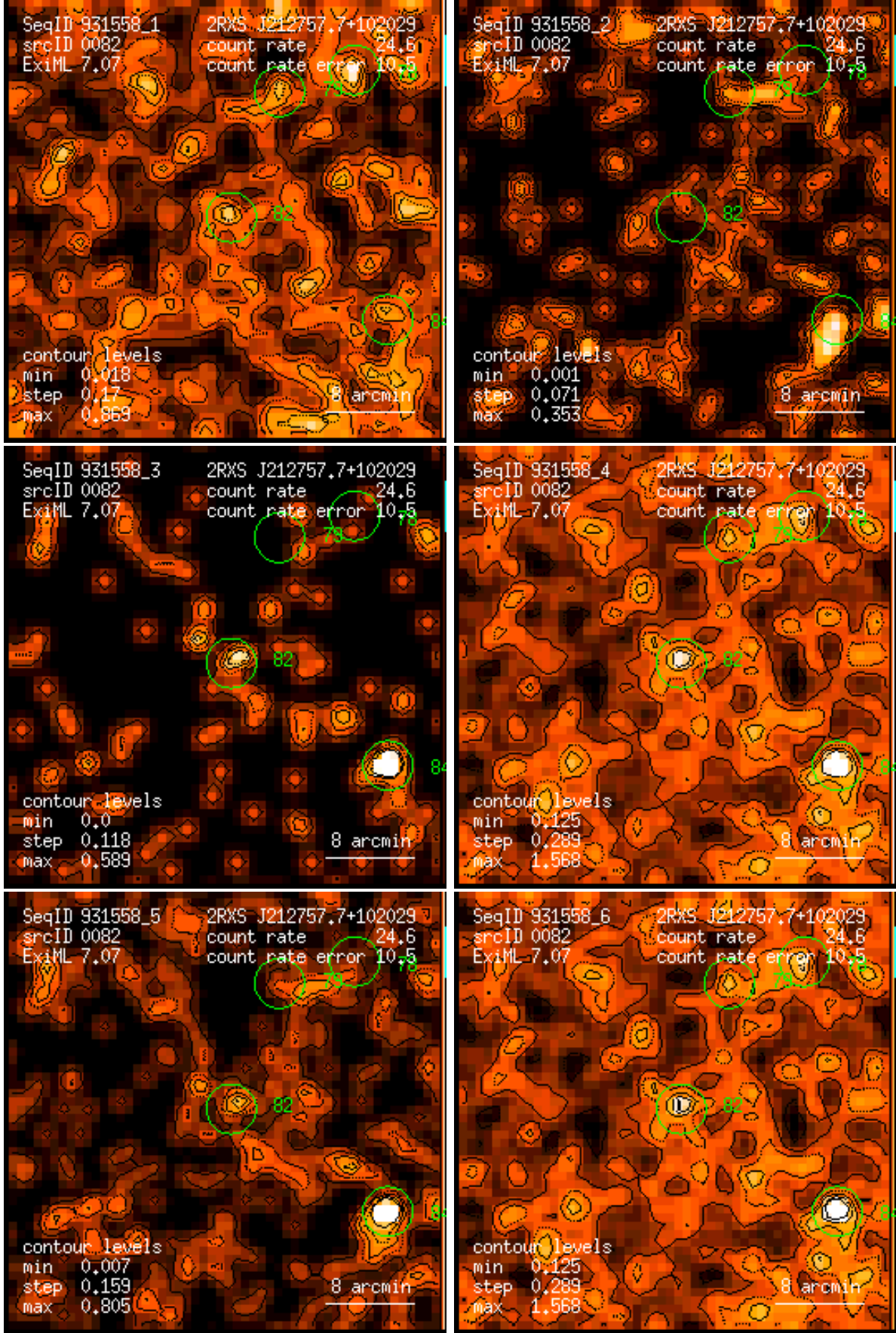
Figure 82: RASS 931558: detection 0082: band rate images, Gaussian filter: (1) PSPC channels 11 – 41, (2) 52 – 90, (3) 91 – 201, (4) 11 – 235, (5) 52 – 201, (6) 11 – 201. Broad band rates in counts/ks. Band rate contour levels in counts/ks/arcmin 2 .
