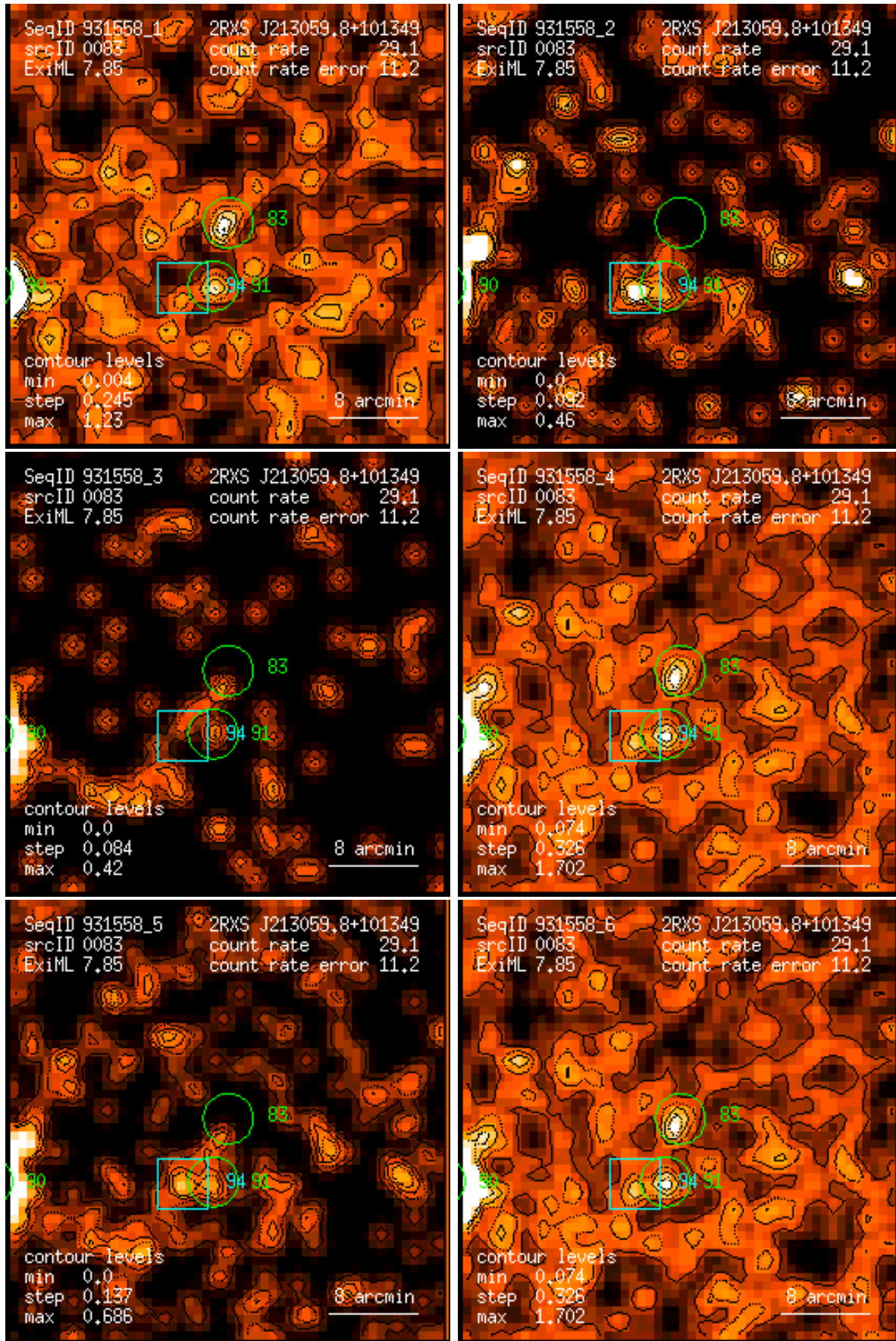
Figure 83: RASS 931558: detection 0083: band rate images, Gaussian filter: (1) PSPC channels 11 – 41, (2) 52 – 90, (3) 91 – 201, (4) 11 – 235, (5) 52 – 201, (6) 11 – 201. Broad band rates in counts/ks. Band rate contour levels in counts/ks/arcmin 2 .
