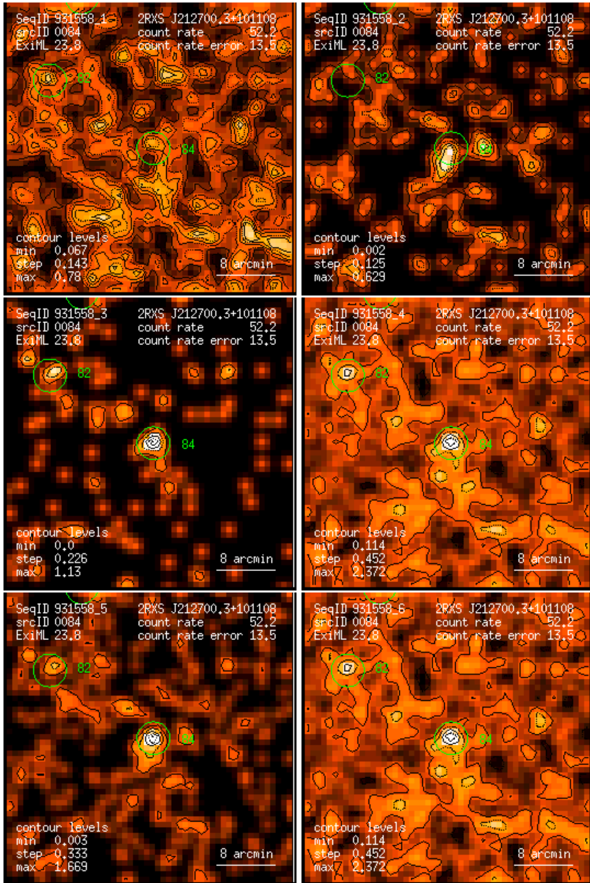
Figure 84: RASS 931558: detection 0084: band rate images, Gaussian filter: (1) PSPC channels 11 – 41, (2) 52 – 90, (3) 91 – 201, (4) 11 – 235, (5) 52 – 201, (6) 11 – 201. Broad band rates in counts/ks. Band rate contour levels in counts/ks/arcmin 2 .
