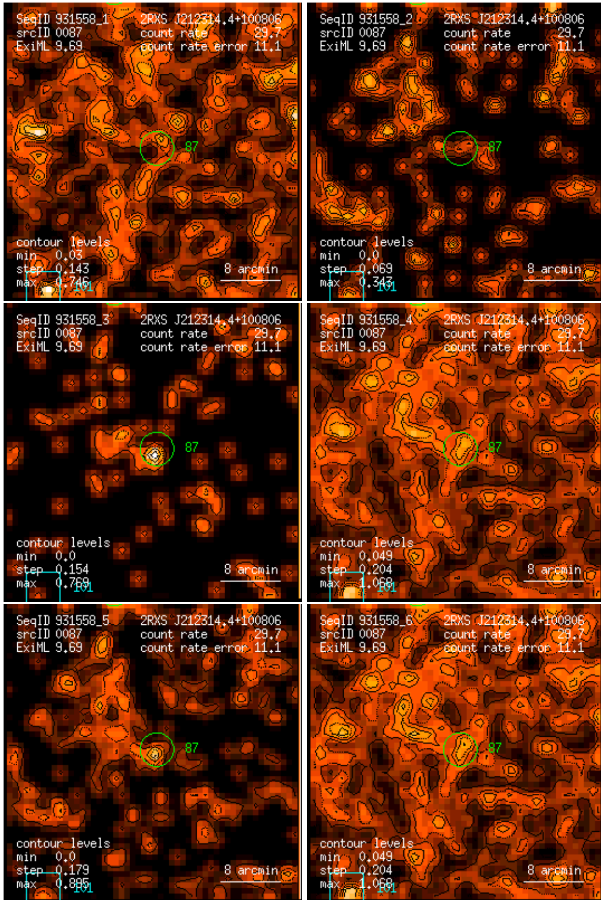
Figure 87: RASS 931558: detection 0087: band rate images, Gaussian filter: (1) PSPC channels 11 – 41, (2) 52 – 90, (3) 91 – 201, (4) 11 – 235, (5) 52 – 201, (6) 11 – 201. Broad band rates in counts/ks. Band rate contour levels in counts/ks/arcmin 2 .
