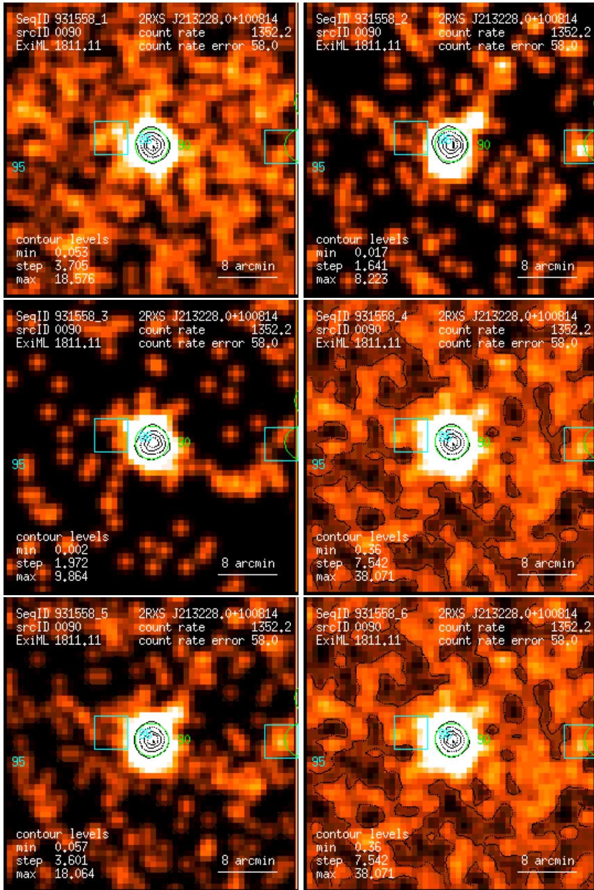
Figure 90: RASS 931558: detection 0090: band rate images, Gaussian filter: (1) PSPC channels 11 – 41, (2) 52 – 90, (3) 91 – 201, (4) 11 – 235, (5) 52 – 201, (6) 11 – 201. Broad band rates in counts/ks. Band rate contour levels in counts/ks/arcmin 2 .
