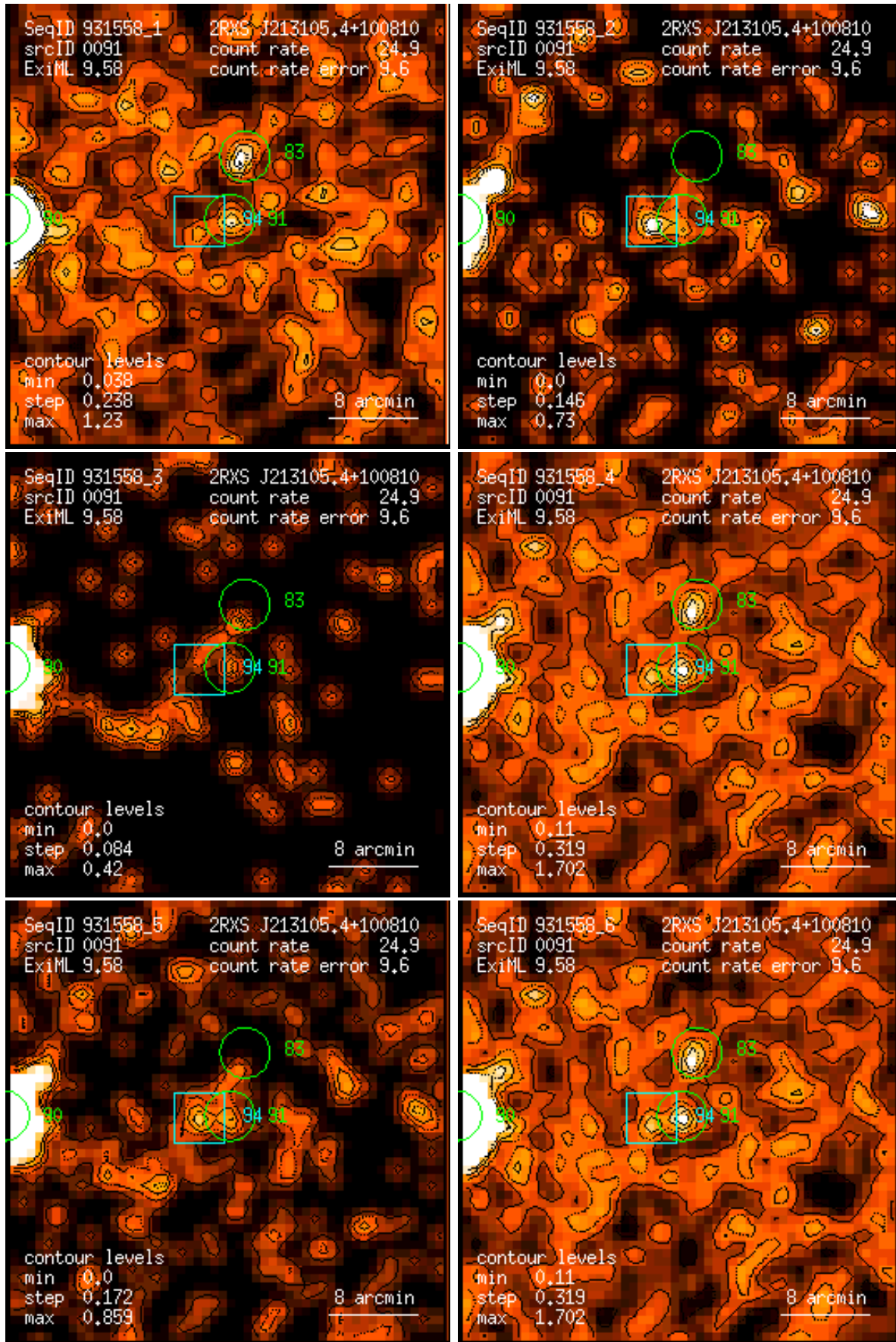
Figure 91: RASS 931558: detection 0091: band rate images, Gaussian filter: (1) PSPC channels 11 – 41, (2) 52 – 90, (3) 91 – 201, (4) 11 – 235, (5) 52 – 201, (6) 11 – 201. Broad band rates in counts/ks. Band rate contour levels in counts/ks/arcmin 2 .
