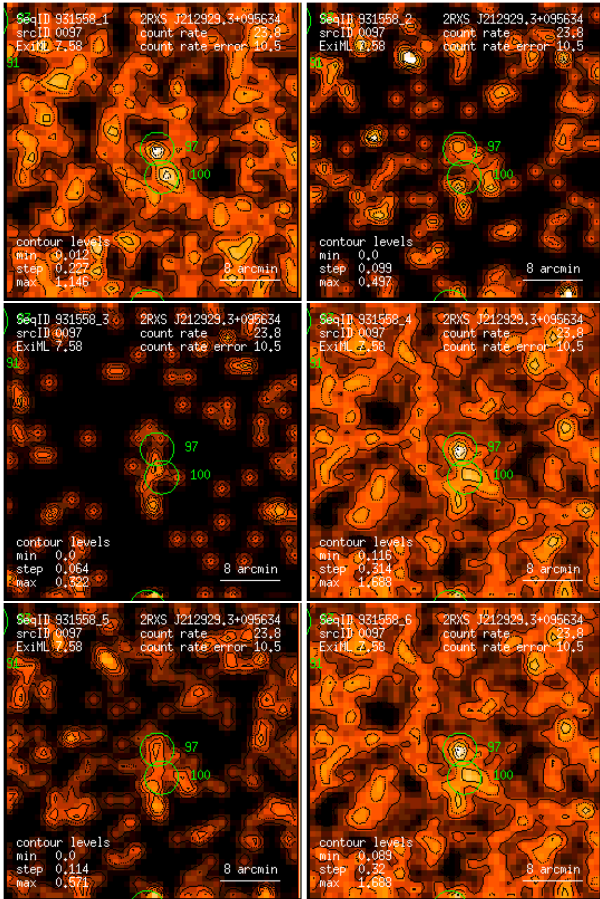
Figure 97: RASS 931558: detection 0097: band rate images, Gaussian filter: (1) PSPC channels 11 – 41, (2) 52 – 90, (3) 91 – 201, (4) 11 – 235, (5) 52 – 201, (6) 11 – 201. Broad band rates in counts/ks. Band rate contour levels in counts/ks/arcmin 2 .
