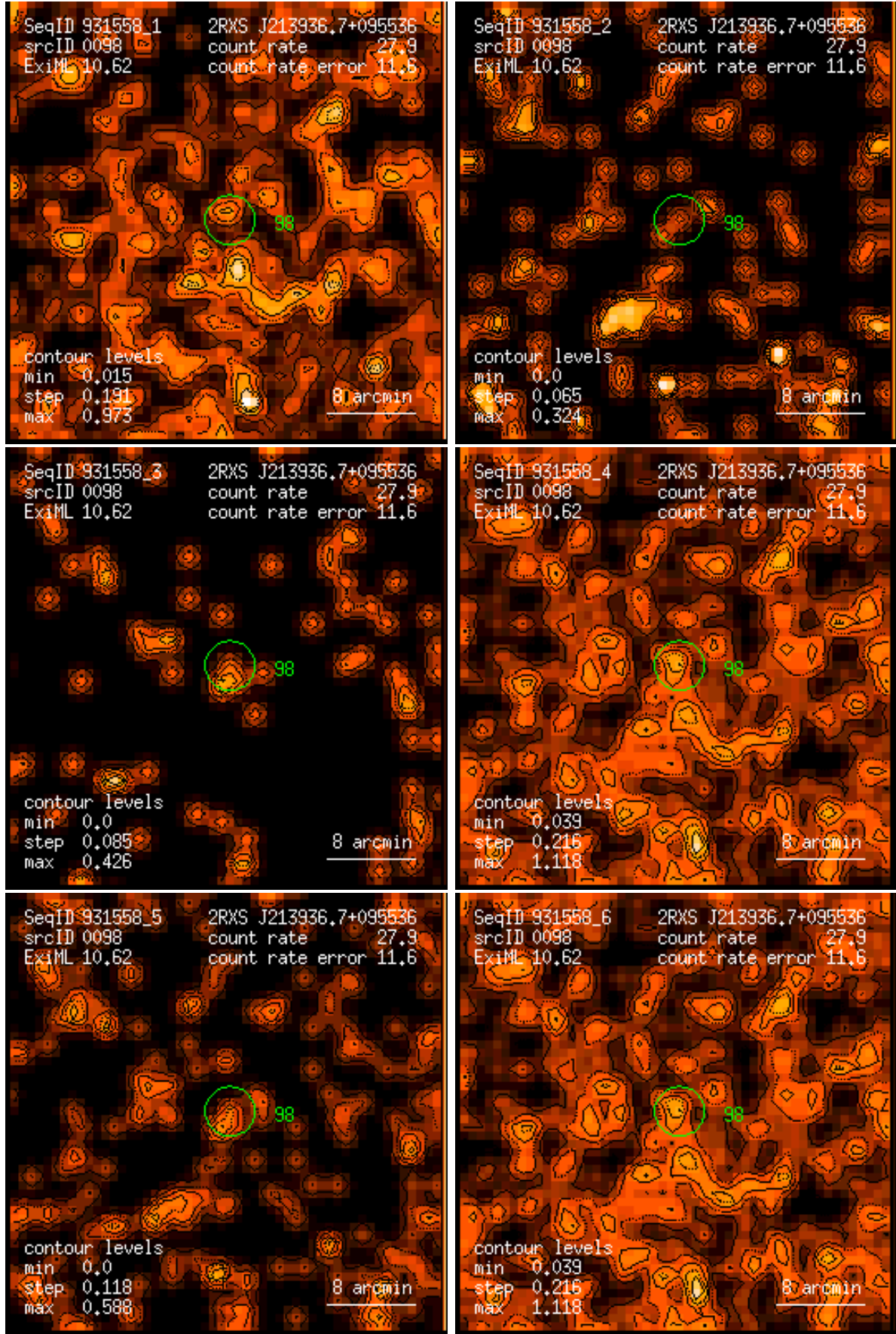
Figure 98: RASS 931558: detection 0098: band rate images, Gaussian filter: (1) PSPC channels 11 – 41, (2) 52 – 90, (3) 91 – 201, (4) 11 – 235, (5) 52 – 201, (6) 11 – 201. Broad band rates in counts/ks. Band rate contour levels in counts/ks/arcmin 2 .
