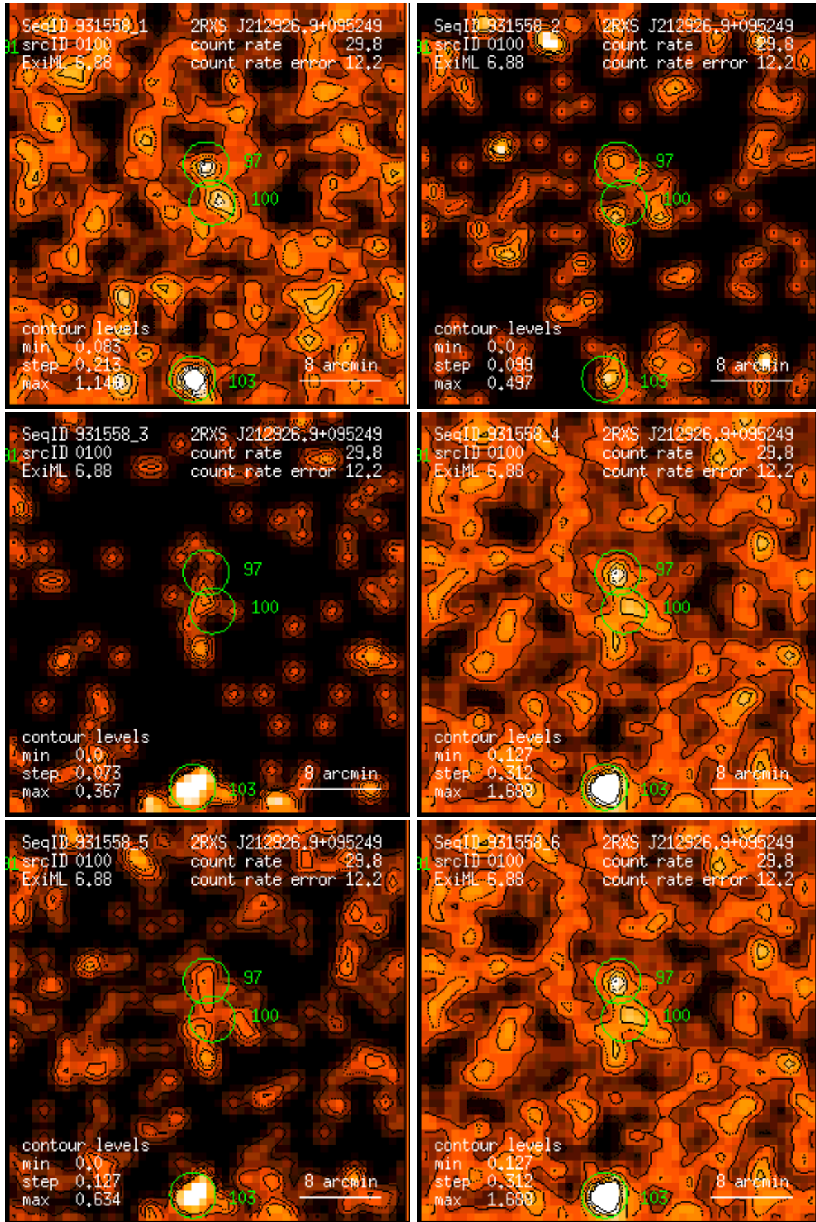
Figure 100: RASS 931558: detection 0100: band rate images, Gaussian filter: (1) PSPC channels 11 – 41, (2) 52 – 90, (3) 91 – 201, (4) 11 – 235, (5) 52 – 201, (6) 11 – 201. Broad band rates in counts/ks. Band rate contour levels in counts/ks/arcmin 2 .
