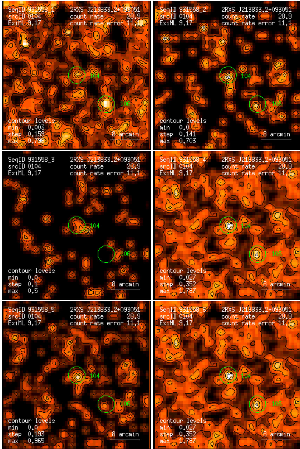
Figure 104: RASS 931558: detection 0104: band rate images, Gaussian filter: (1) PSPC channels 11 – 41, (2) 52 – 90, (3) 91 – 201, (4) 11 – 235, (5) 52 – 201, (6) 11 – 201. Broad band rates in counts/ks. Band rate contour levels in counts/ks/arcmin 2 .
