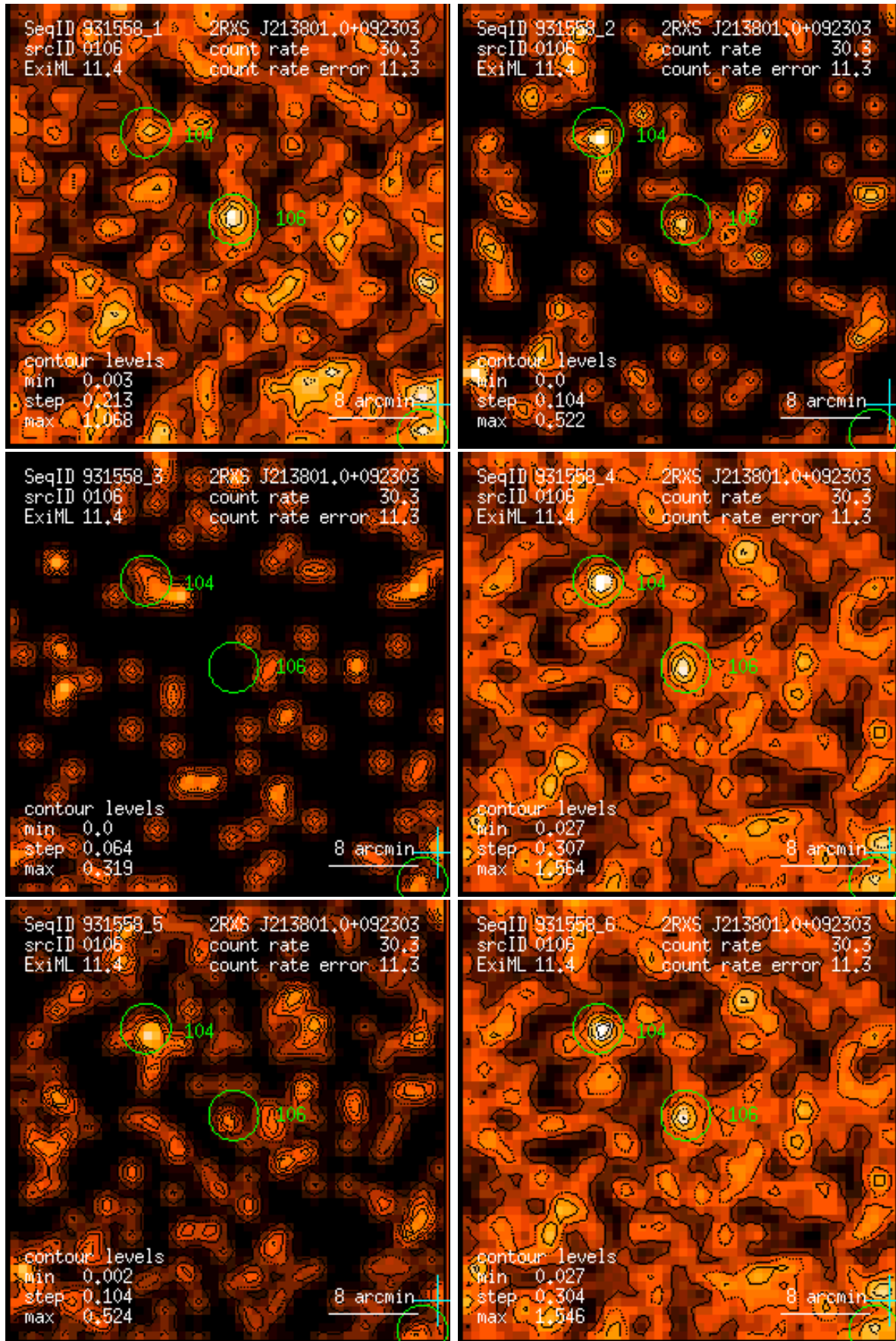
Figure 106: RASS 931558: detection 0106: band rate images, Gaussian filter: (1) PSPC channels 11 – 41, (2) 52 – 90, (3) 91 – 201, (4) 11 – 235, (5) 52 – 201, (6) 11 – 201. Broad band rates in counts/ks. Band rate contour levels in counts/ks/arcmin 2 .
