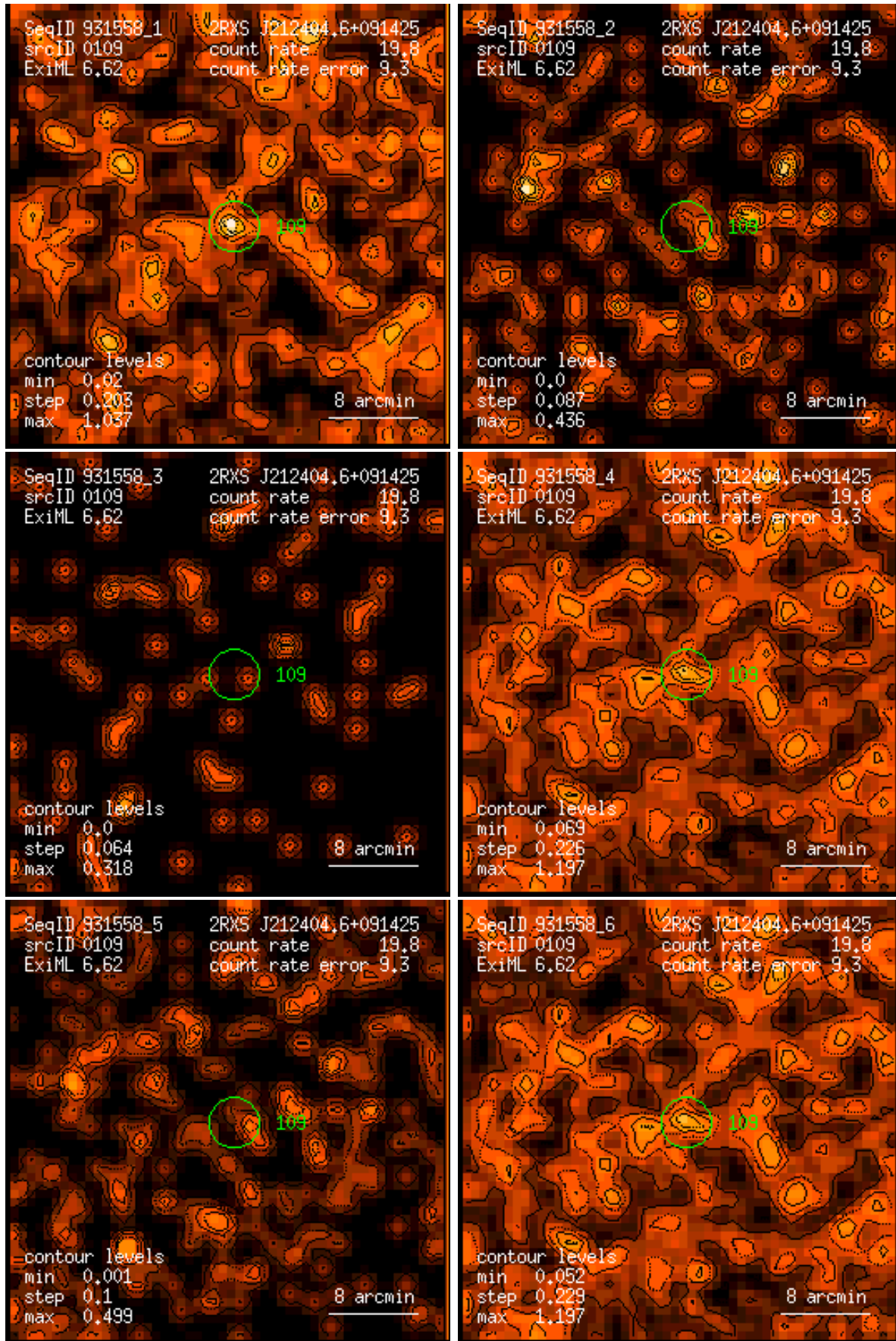
Figure 109: RASS 931558: detection 0109: band rate images, Gaussian filter: (1) PSPC channels 11 – 41, (2) 52 – 90, (3) 91 – 201, (4) 11 – 235, (5) 52 – 201, (6) 11 – 201. Broad band rates in counts/ks. Band rate contour levels in counts/ks/arcmin 2 .
