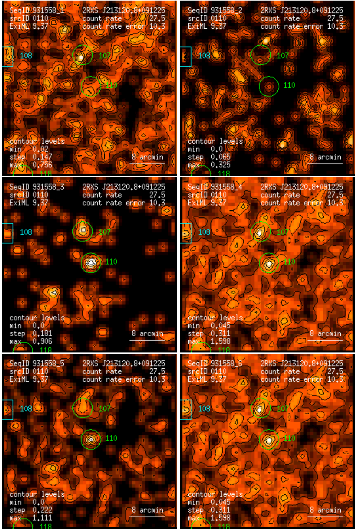
Figure 110: RASS 931558: detection 0110: band rate images, Gaussian filter: (1) PSPC channels 11 – 41, (2) 52 – 90, (3) 91 – 201, (4) 11 – 235, (5) 52 – 201, (6) 11 – 201. Broad band rates in counts/ks. Band rate contour levels in counts/ks/arcmin 2 .
